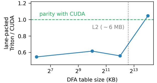
Figure 3. The residual is regime-dependent. Lane-packed Triton trails CUDA by ~1.7× while the DFA table is cache-resident and reaches parity (1.05×) once a 16 MB table spills past L2, where both must hide latency across warps.
