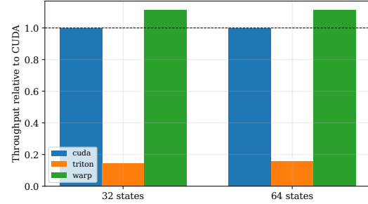
Fig. 1. Throughput relative to CUDA : Triton (tile) \ll Warp (thread) \approx CUDA . Regret is the execution paradigm, not abstraction height.
