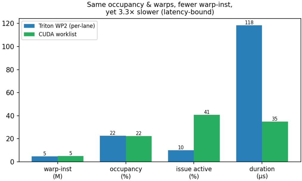
Fig. 3. Per-lane Triton vs. CUDA (16384 strings, 32 states): same occupancy, fewer warp-instructions, yet 3.3× slower at 9.9% vs. 41% issue activity: latency-bound.
