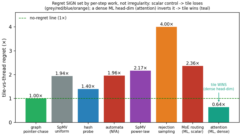
Fig. 7. The regret law across eight oracle-gated irregular workloads, by dominant mechanism. A graph pointer-chase (green) is the negative control (irregular memory + dependent loads, no control divergence \Rightarrow regret 1.00 \times ). Regret grows with scalar control / divergence (grey, red, blue, orange), peaking at 4 \times . The two ML witnesses (right) test the sign : MoE routing (scalar per step) confirms the law (2.36 \times ), while ragged attention (dense head-dim) inverts it (0.64 \times , teal, below the no-regret line; the tile wins), because per-step instruction efficiency, not irregularity, sets the sign.
