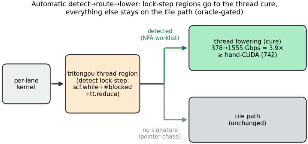
Fig. 8. The automatic detect→route→lower loop (P2). The detection pass (in libtriton) matches the lock-step signature; the lock-step NFA workload is routed to the thread lowering (378→1555 Gbps = 3.9×, exceeding hand-CUDA), while a no-signature kernel (pointer-chase) stays on the tile path. All routing oracle-gated; numbers from the versioned CSVs.
