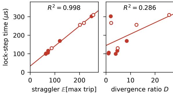
Figure 5. The lock-step cost is set by the absolute straggler, not by the divergence ratio . Ten trip distributions, filled markers designed, open markers held out. A one-parameter fit on the straggler explains the cost; the same fit on D = \mathbb{E}[\max \text{trip}] / \mathbb{E}[\text{trip}] does not.
