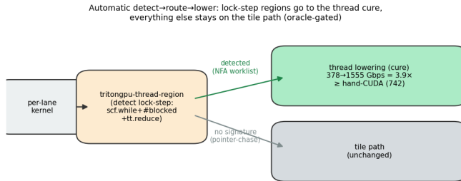
Fig. 8. The automatic detect→route→lower loop (P2). The detection pass (in libtriton ) matches the lock-step signature; the lock-step NFA worklist is routed to the thread lowering ( 378\rightarrow 1555 Gbps = 3.9\times , exceeding hand-CUDA), while a no-signature kernel (pointer-chase) stays on the tile path. All routing oracle-gated; numbers from the versioned CSVs.
