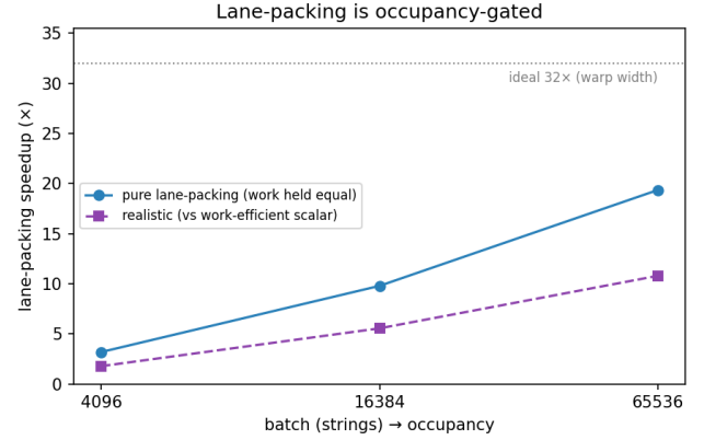
Figure 2. Lane-packing’s benefit is occupancy-gated: the pure-packing speedup 3.2\times \rightarrow 19.4\times with batch (toward the ideal 32\times ) as more warps fill the GPU.
