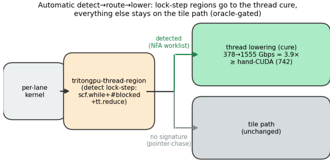
Fig. 8. The automatic detect→route→lower loop (P2). The detection pass (in libtriton) matches the lock-step signature; the lock-step NFA worklist is routed to the thread lowering (378→1555 Gbps = 3.9×, exceeding hand-CUDA), while a no-signature kernel (pointer-chase) stays on the tile path. All routing oracle-gated; numbers from the versioned CSVs.
