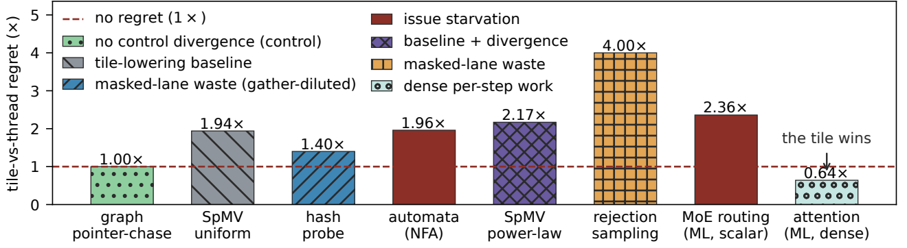
Figure 6. Tile-versus-thread regret across eight oracle-gated irregular witnesses, keyed by dominant mechanism through both fill and hatch. The graph pointer-chase is the negative control: irregular memory and dependent loads with a fixed step count cost nothing at all. Uniform SpMV is the other half of the story: no divergence either, but the tile mapping loses occupancy, so a floor can exist without any control cost. What grows above such a floor is set by per-step scalar control. Ragged attention inverts the sign, because a dense head-dim payload makes the tile issue fewer instructions than the thread model.
