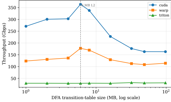
Fig. 2. DFA (memory-bound face), throughput vs table size (log x ), median over 3 random DFAs/size: CUDA/Warp peak at the 6 MB L2 then drop \sim 2.2\times to a DRAM plateau; Triton stays flat (29–32 Gbps)—scalar-gather-bound, never reaching the memory regime.
