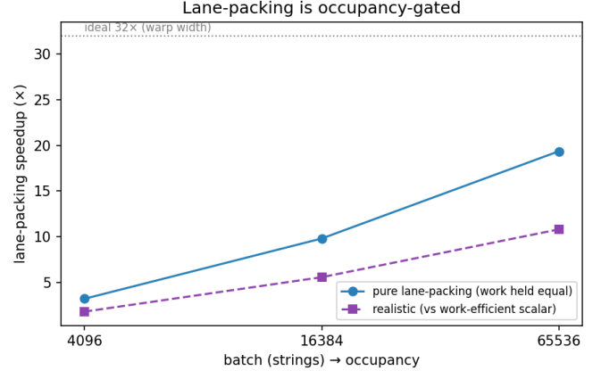
Fig. 2. Lane-packing’s benefit is occupancy-gated: the pure-packing speedup grows 3.2\times \rightarrow 19.4\times with batch (toward the ideal 32\times ) as more warps fill the GPU.
