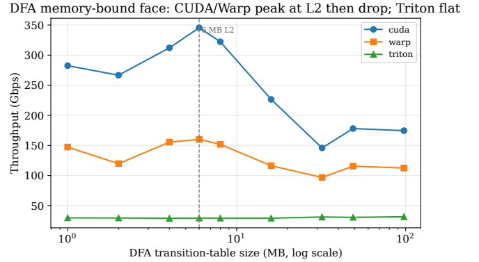
Fig. 6. DFA (memory-bound face), throughput vs table size (log x ): CUDA/Warp peak at the 6 MB L2 then drop 2.4 \times to a DRAM plateau; Triton stays flat (29–32 Gbps)—scalar-gather-bound, never reaching the memory regime.
