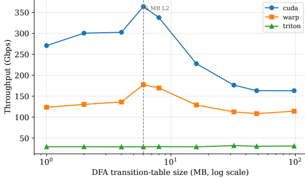
DFA memory-bound face: CUDA/Warp peak at L2 then drop; Triton flat
