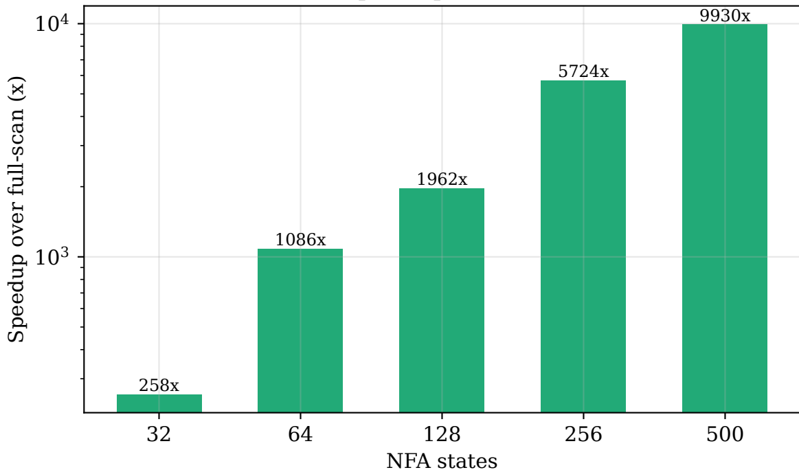
Work-efficient worklist speedup over O(n^2) full-scan (CUDA)
