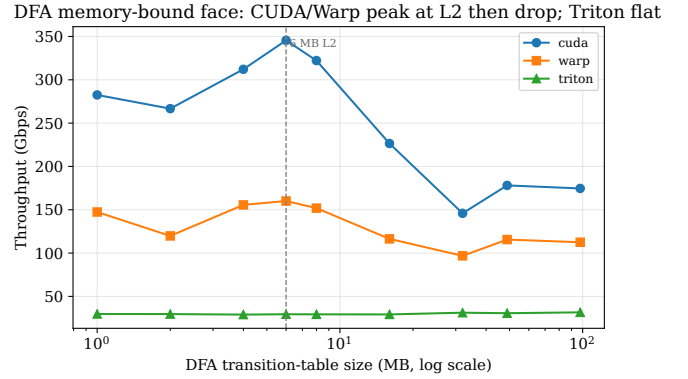
Fig. 6. DFA (memory-bound face), throughput vs table size (log x ): CUDA/Warp peak at the 6 MB L2 then drop 2.4× to a DRAM plateau; Triton stays flat (29–32 Gbps)—scalar-gather-bound, never reaching the memory regime.
