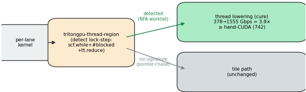
Fig. 8. The automatic detect \rightarrow route \rightarrow lower loop (P2). The detection pass (in libtriton) matches the lock-step signature; the lock-step NFA worklist is routed to the thread lowering (378 \rightarrow 1555 Gbps = 3.9 \times , exceeding hand-CUDA), while a no-signature kernel (pointer-chase) stays on the tile path. All routing oracle-gated; numbers from the versioned CSVs.
