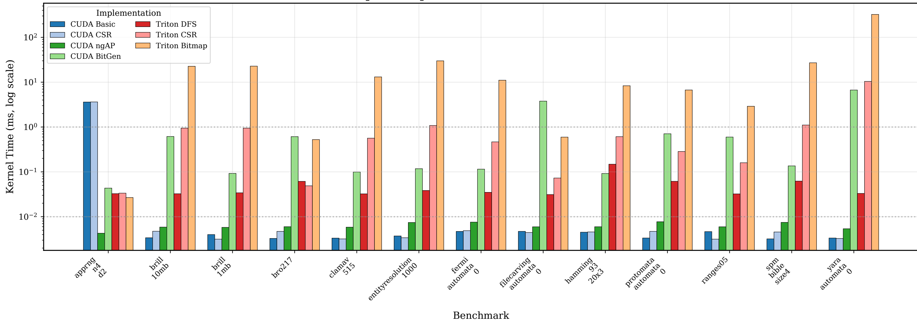
FSM Techniques Comparison: CUDA vs Triton (All Benchmarks)
