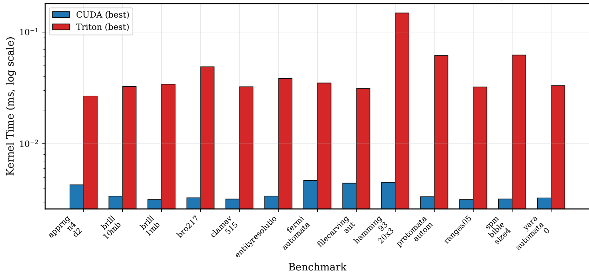
FSM Kernel Time: CUDA vs Triton (Triton 10x slower median)
