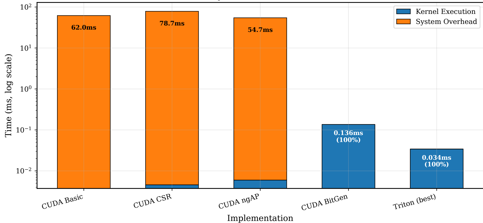
Kernel Time vs System Overhead (FSM Workloads)
