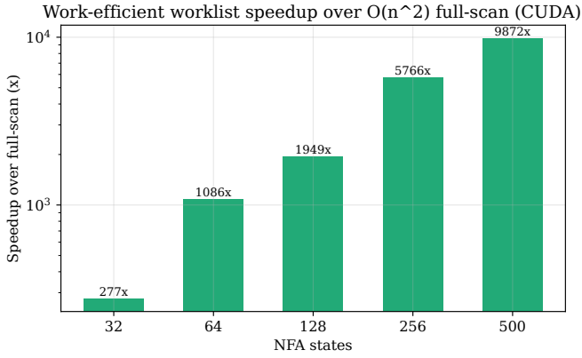
Fig. 2. Work-efficient worklist speedup over O(n^2) full-scan (CUDA), growing with state count.
