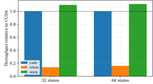
Fig. 4. Throughput relative to CUDA: Triton (tile) \ll Warp (thread) \approx CUDA. Regret is the execution paradigm, not abstraction height.
