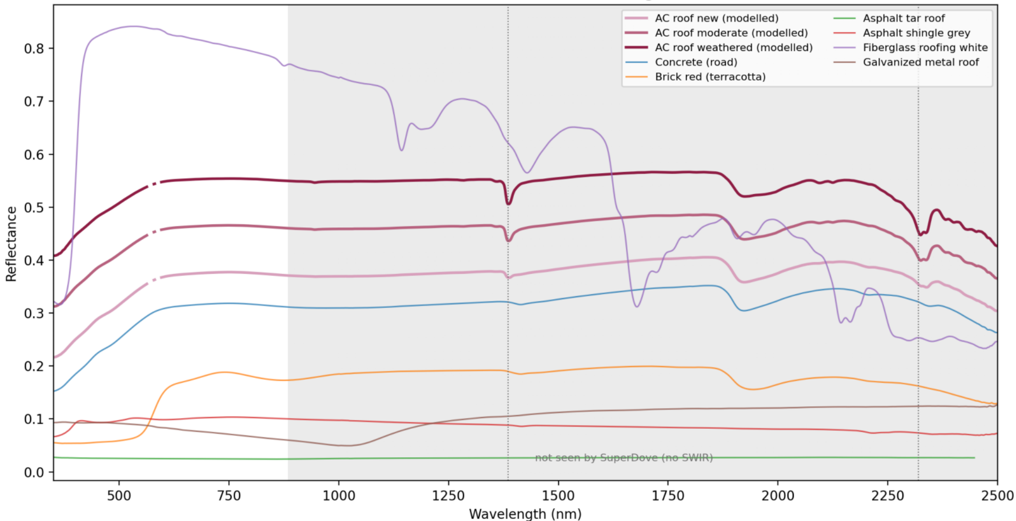
Asbestos-cement roof (modelled, Cilia 2015 mixing) vs roof confusers
