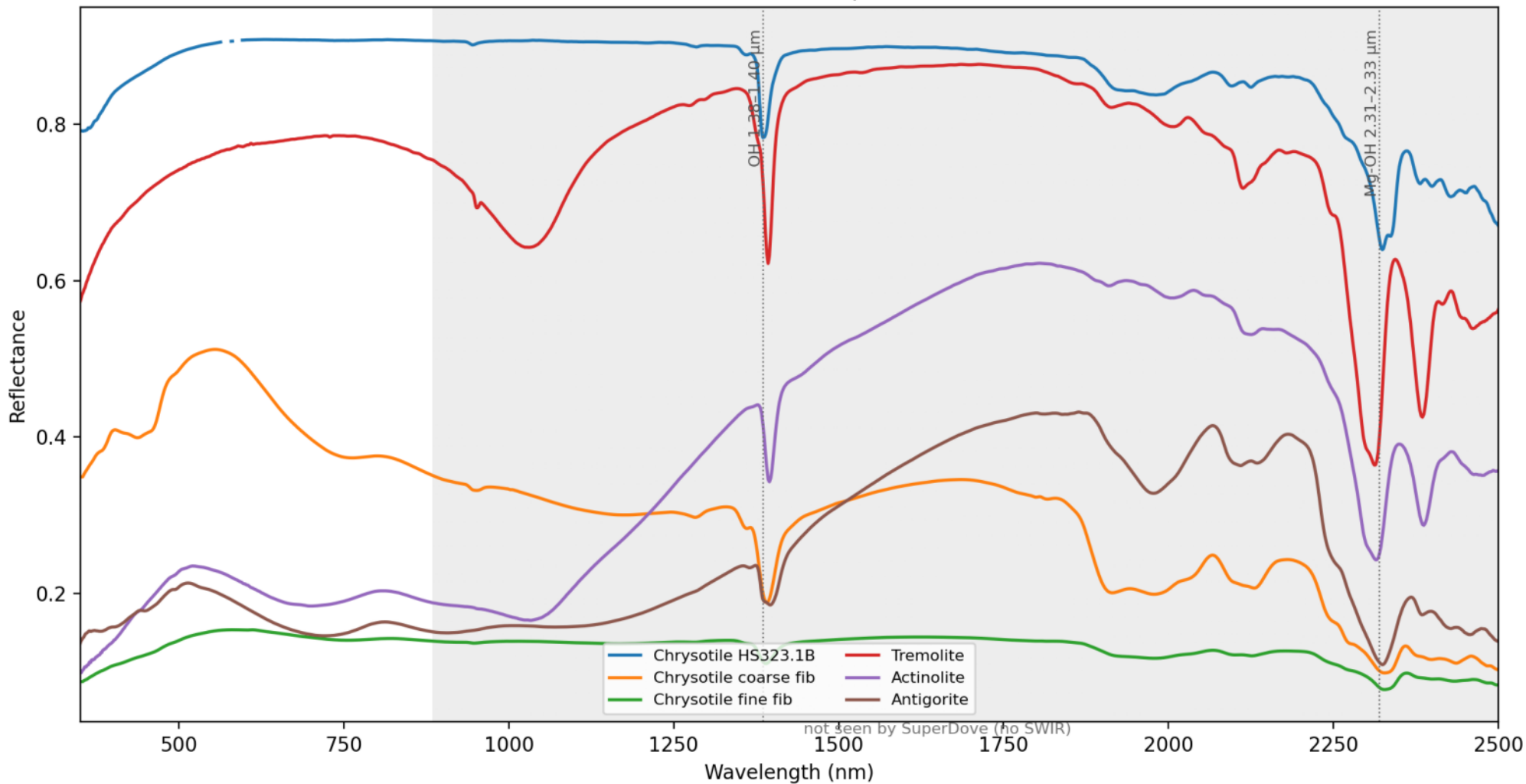
Pure asbestos minerals — USGS splib07a (ASD, 2151 ch)
