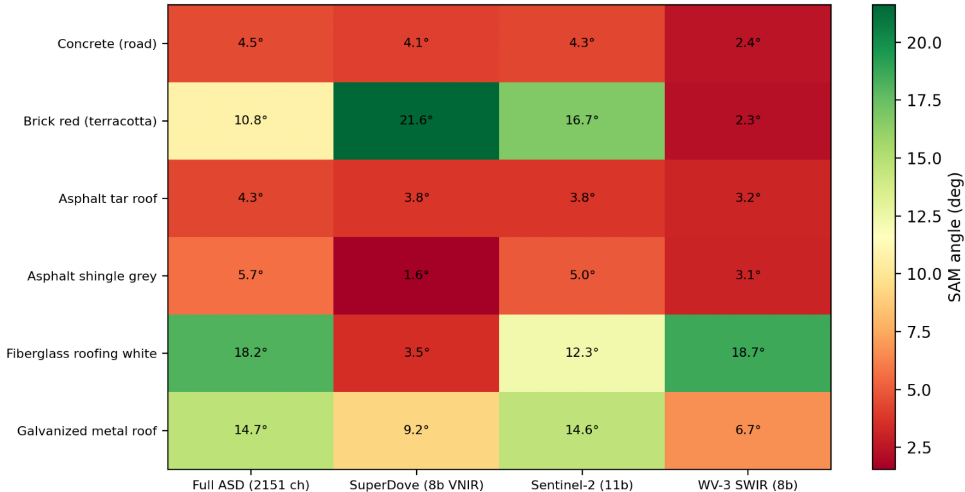
SAM separability: 'AC roof weathered' vs confusers (higher = more separable)
