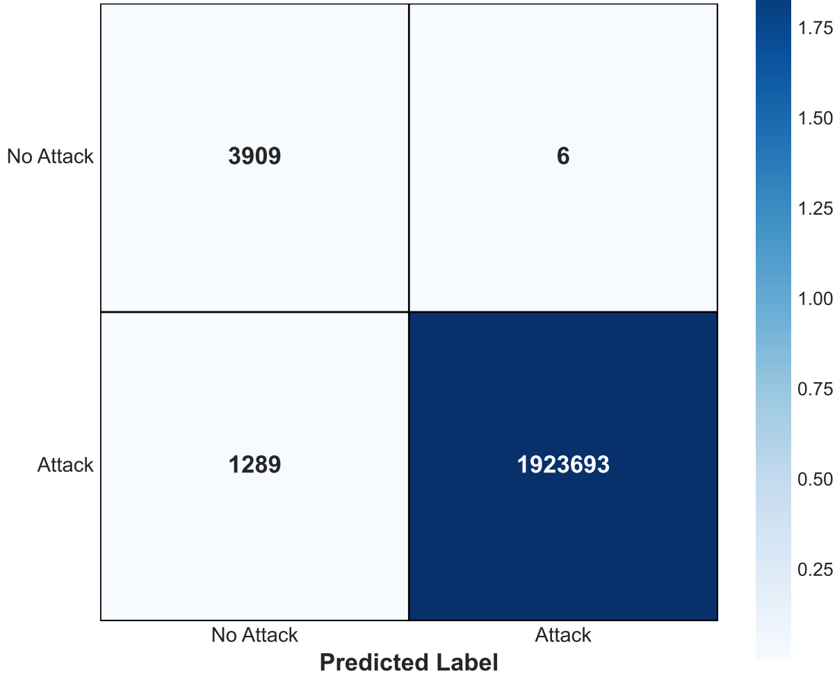
Balanced Baseline MLP Confusion Matrix
