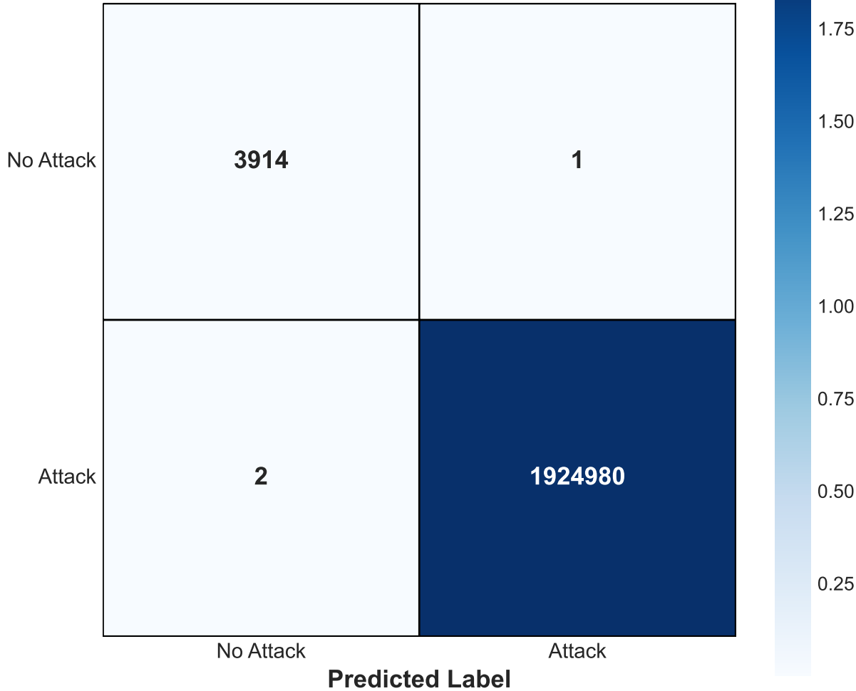
ImbalancedOptuna Optimization RF Confusion Matrix
