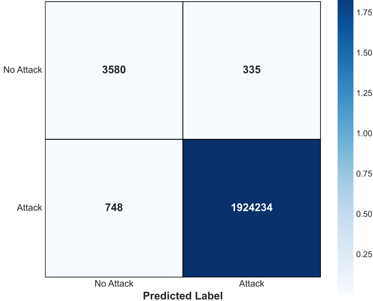
Imbalanced Baseline Logistic Regression Confusion Matrix
