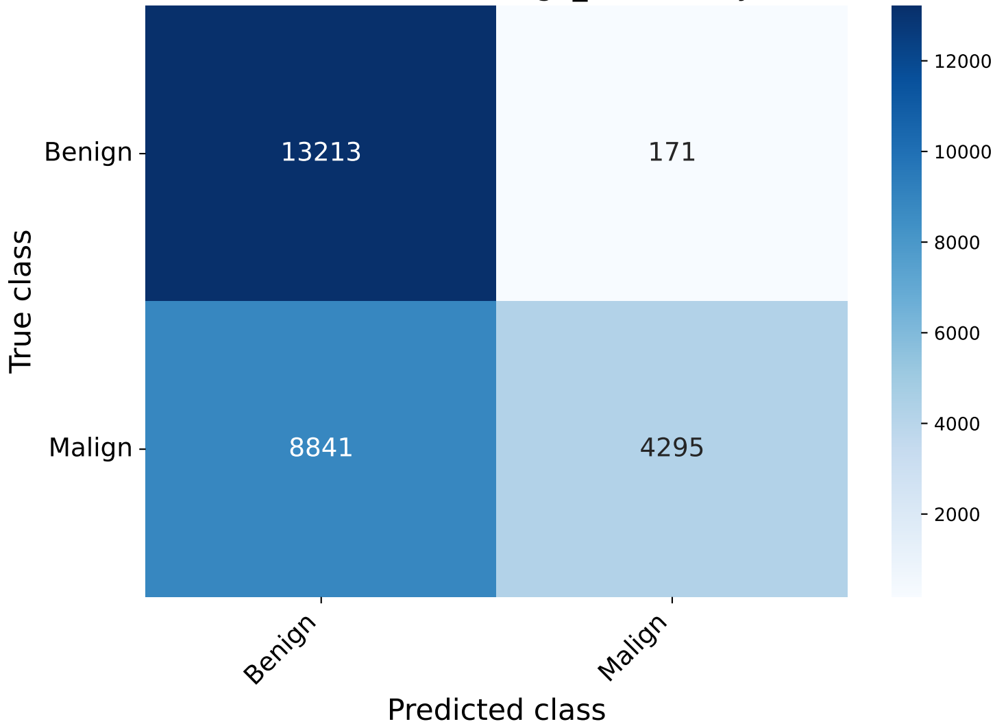
Confusion matrix - xgb_full - binary
