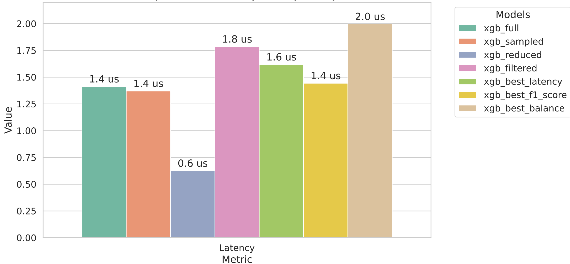
Comparison of Models by Latency (binary)
