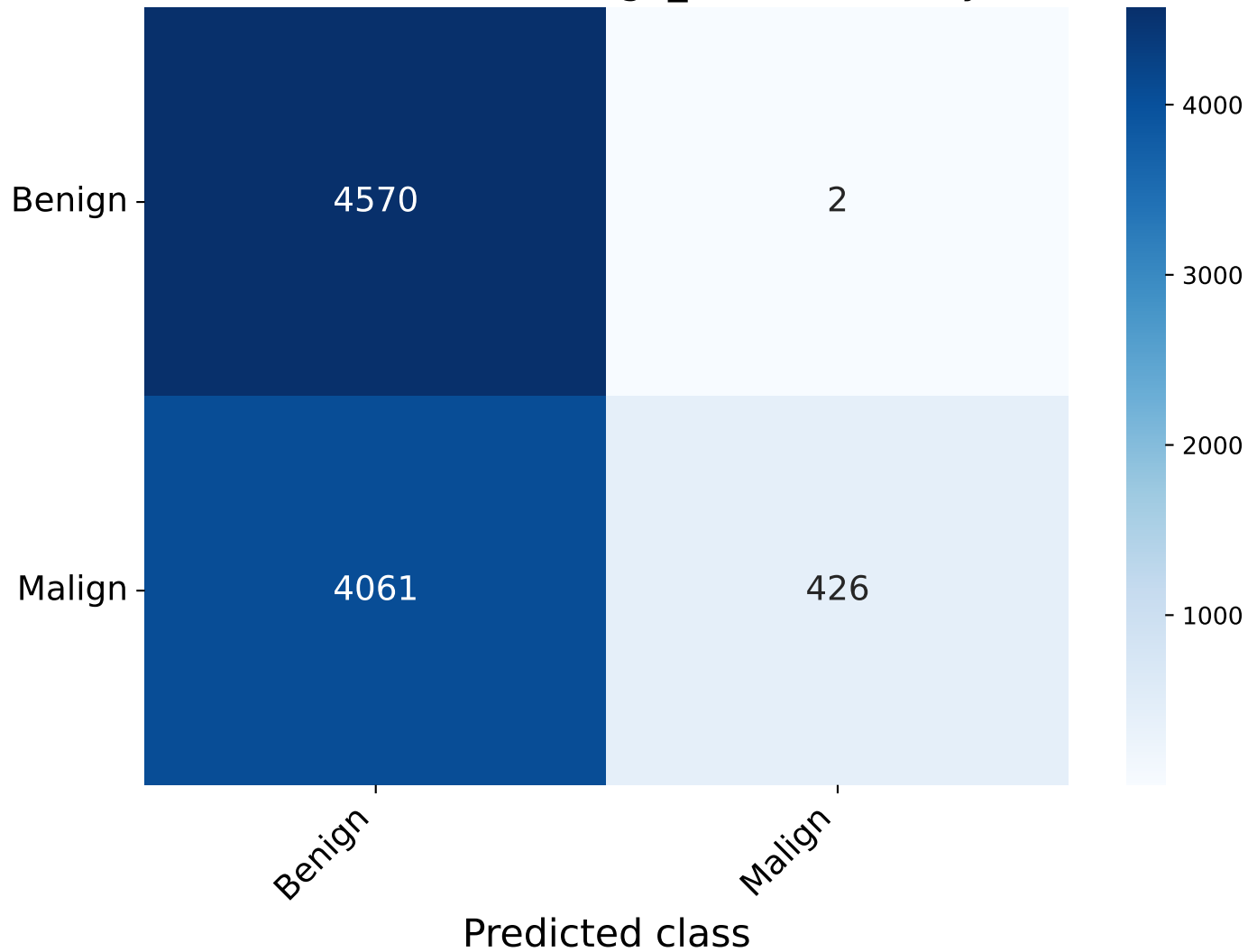
Confusion matrix - xgb_filtered - binary
