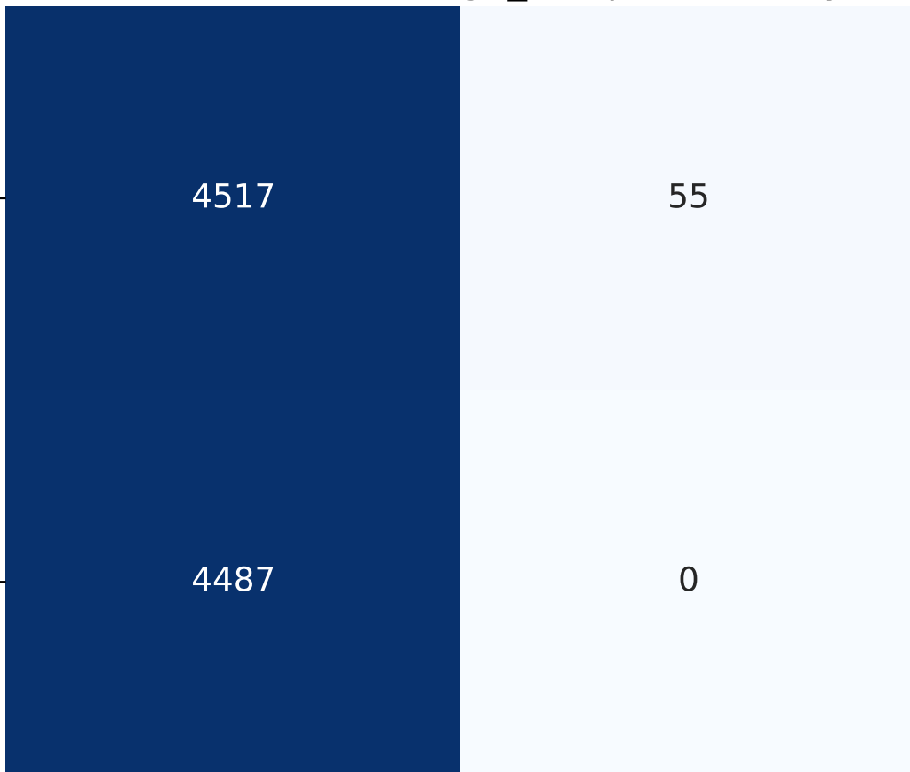
Confusion matrix - xgb_sampled - binary
