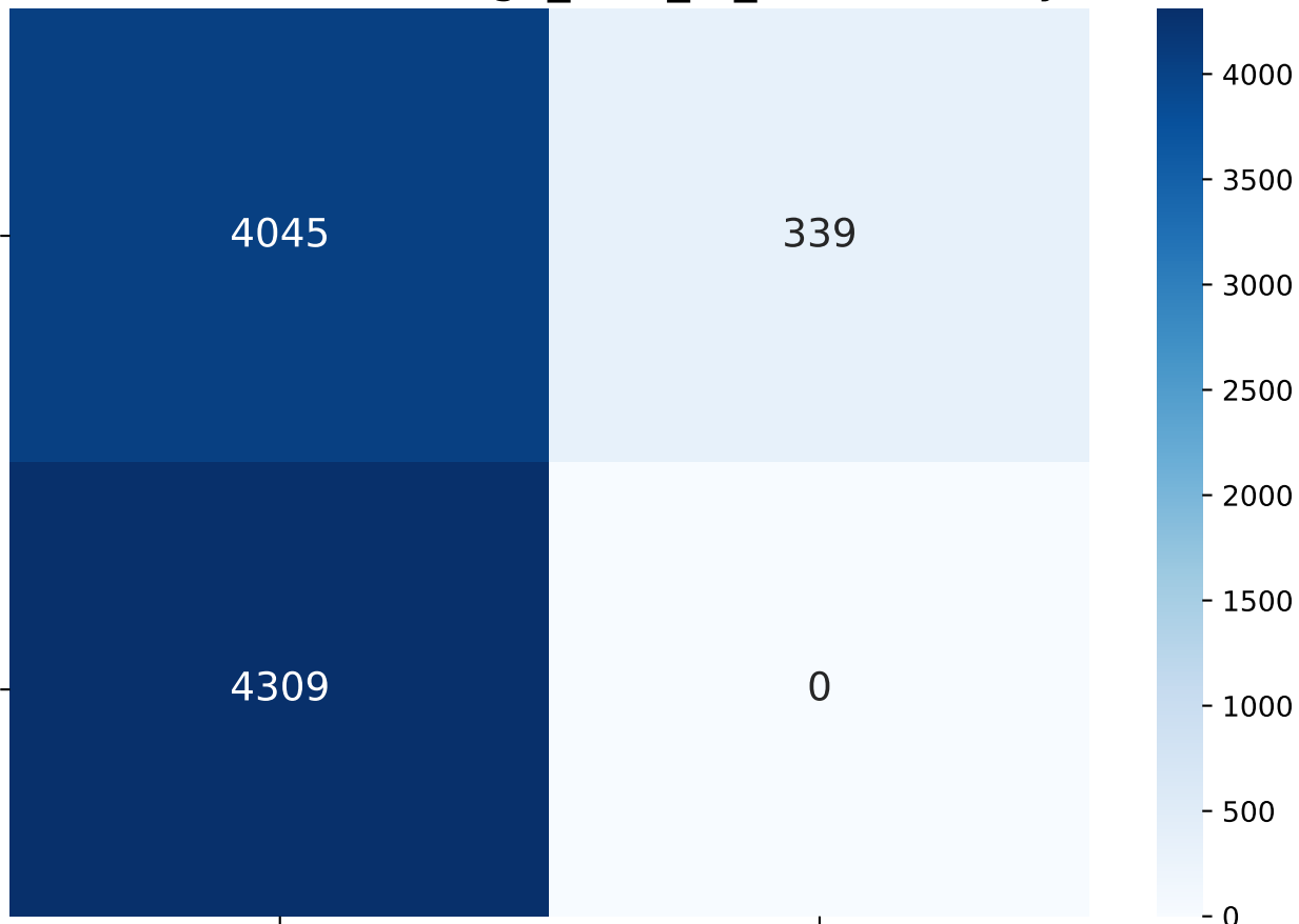
Confusion matrix - xgb_best_f1_score - binary
