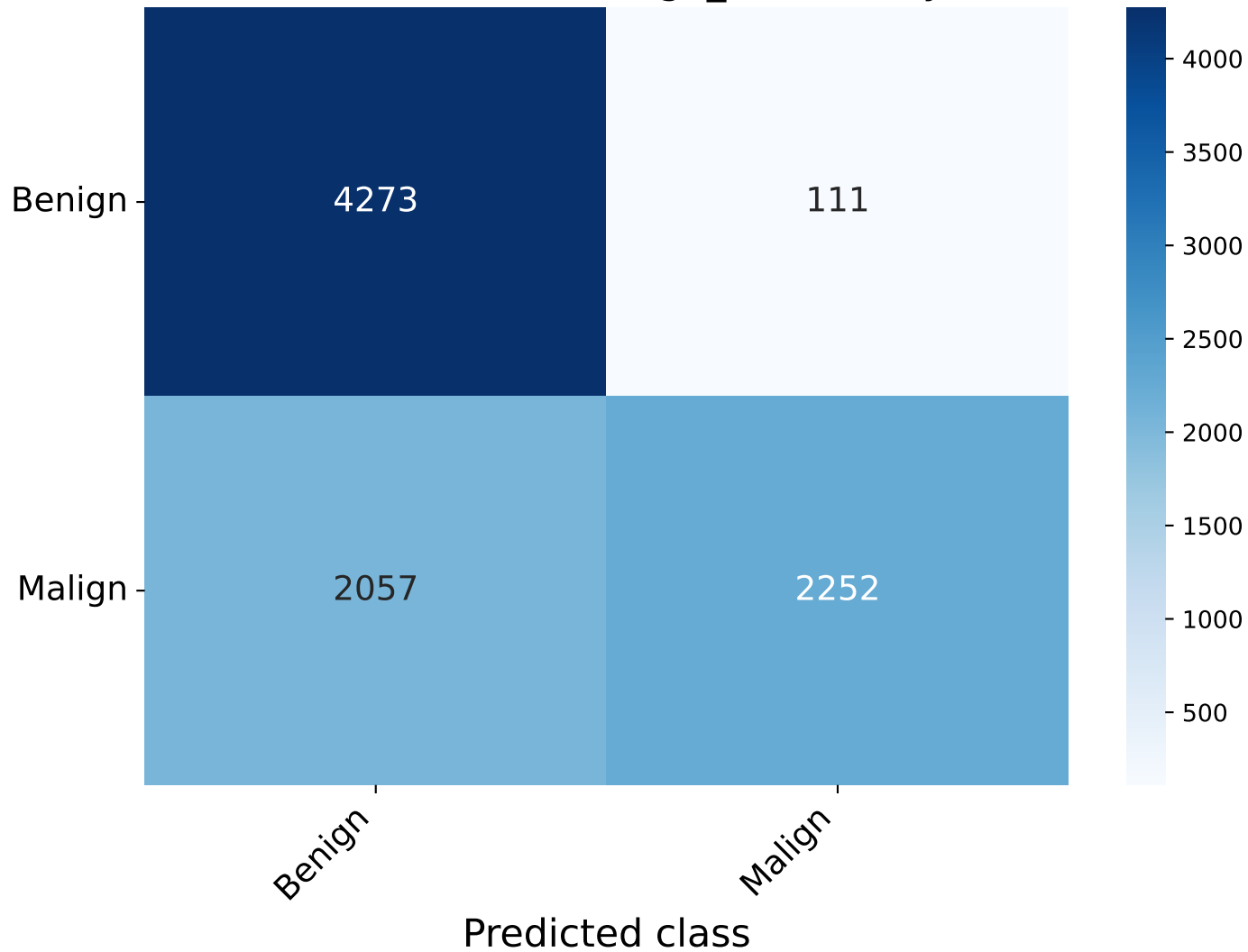
Confusion matrix - xgb_full - binary
