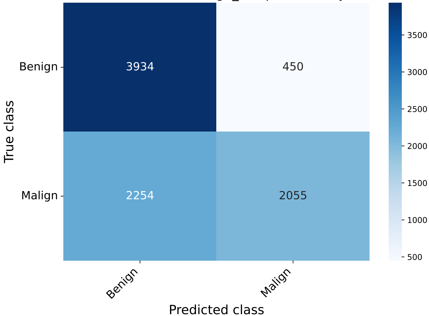
Confusion matrix - xgb_sampled - binary
