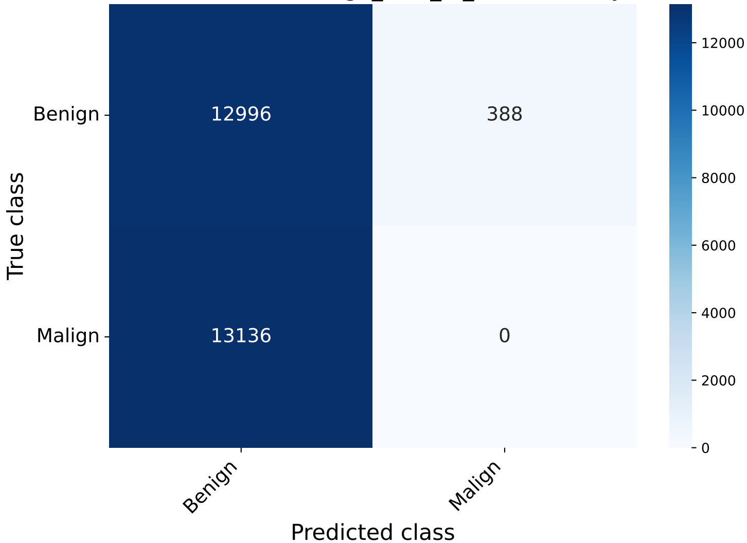
Confusion matrix - xgb_best_f1_score - binary
