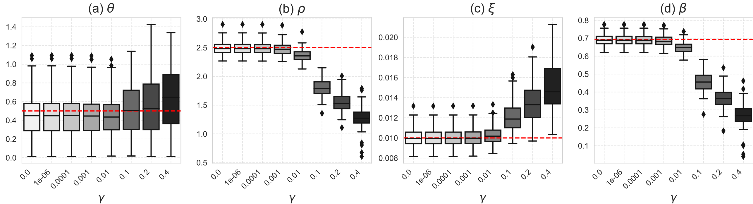
Parameter estimates – (i) Administrative censoring
