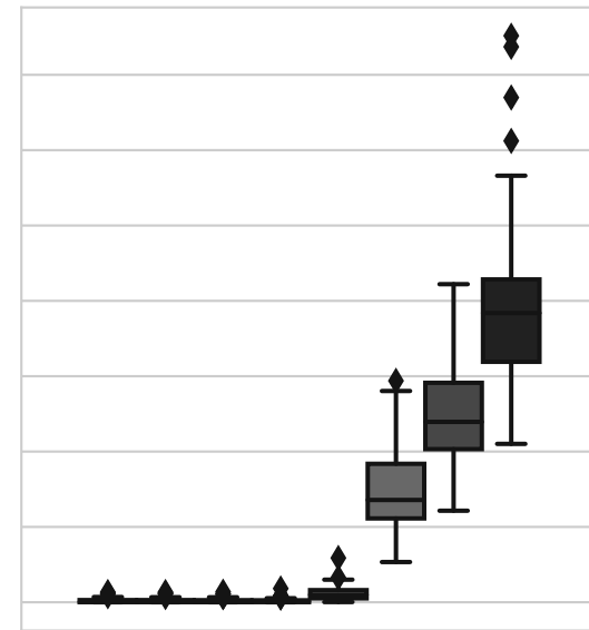
(iv) \beta
