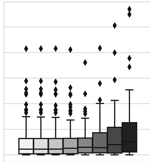
(i) \theta
