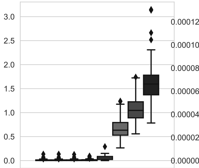
(ii) \rho
