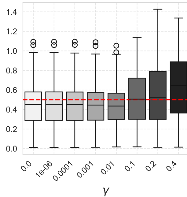
(a) \theta
