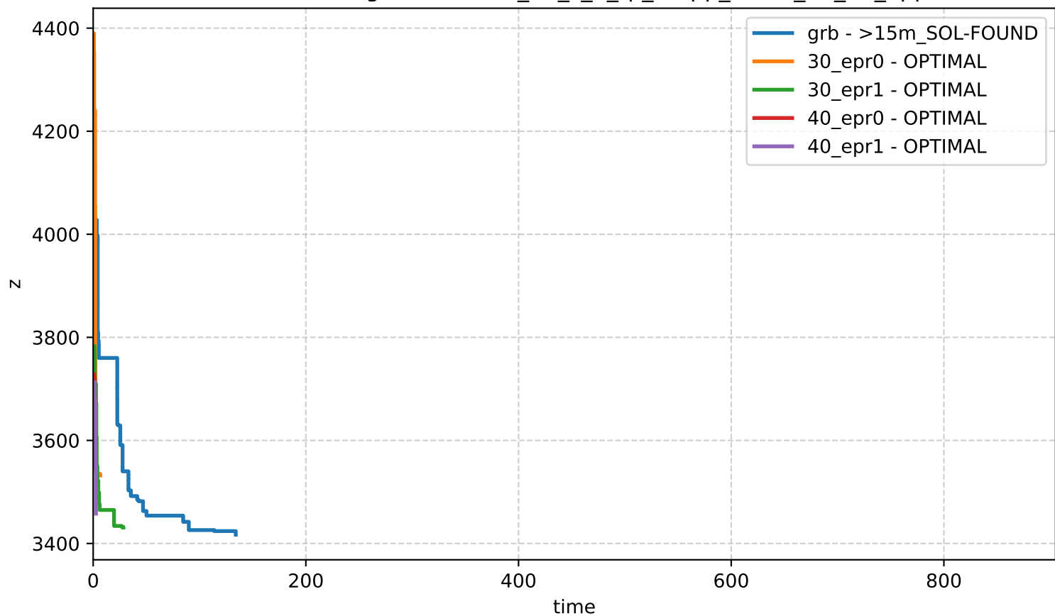
Bound Profiling - network-n_60_s_1_rp_0-app_set-id_18_11_apps
