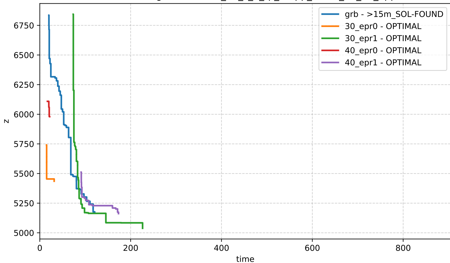
Bound Profiling - network-n_60_s_1_rp_0-app_set-id_41_18_apps
