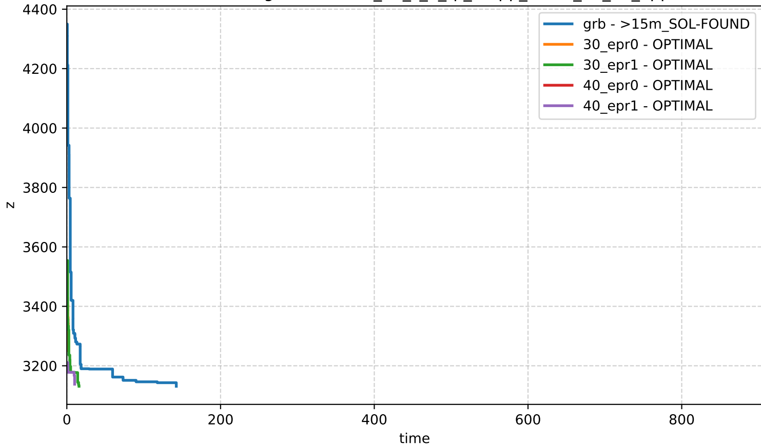
Bound Profiling - network-n_40_s_2_rp_0-app_set-id_24_13_apps
