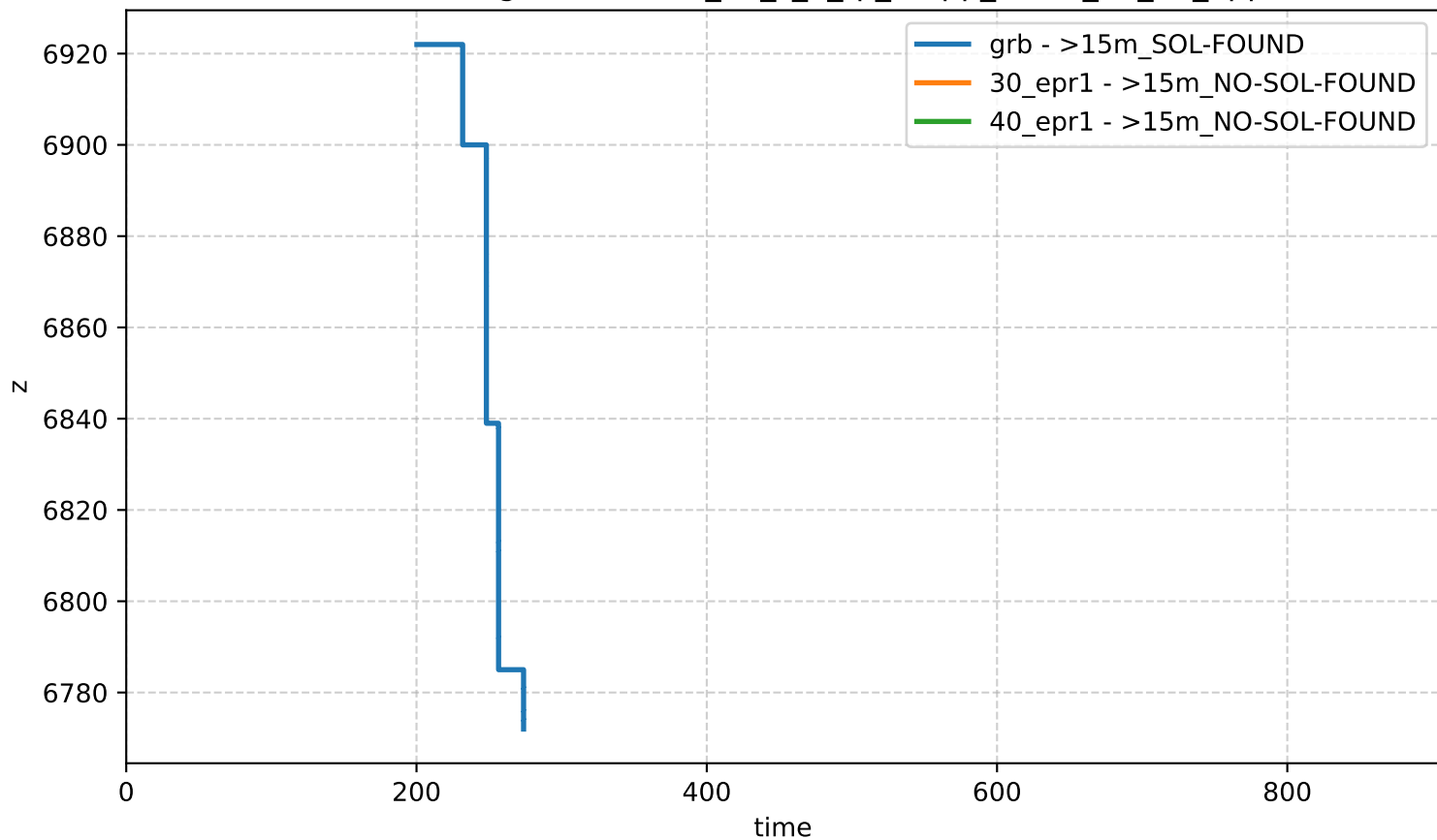
Bound Profiling - network-n_60_s_0_rp_0-app_set-id_52_22_apps
