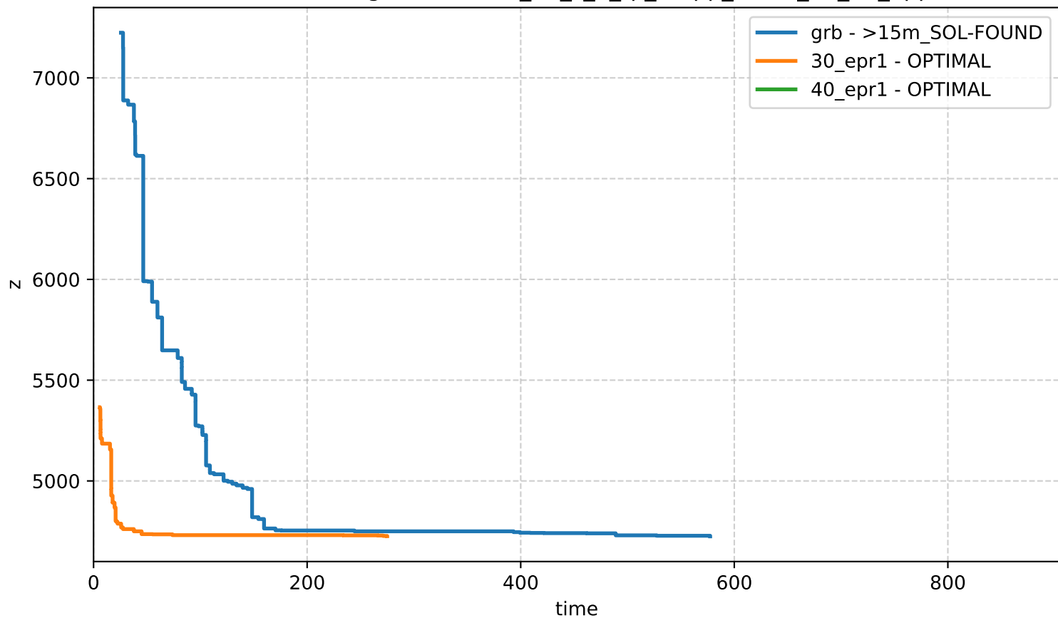
Bound Profiling - network-n_60_s_0_rp_0-app_set-id_51_22_apps
