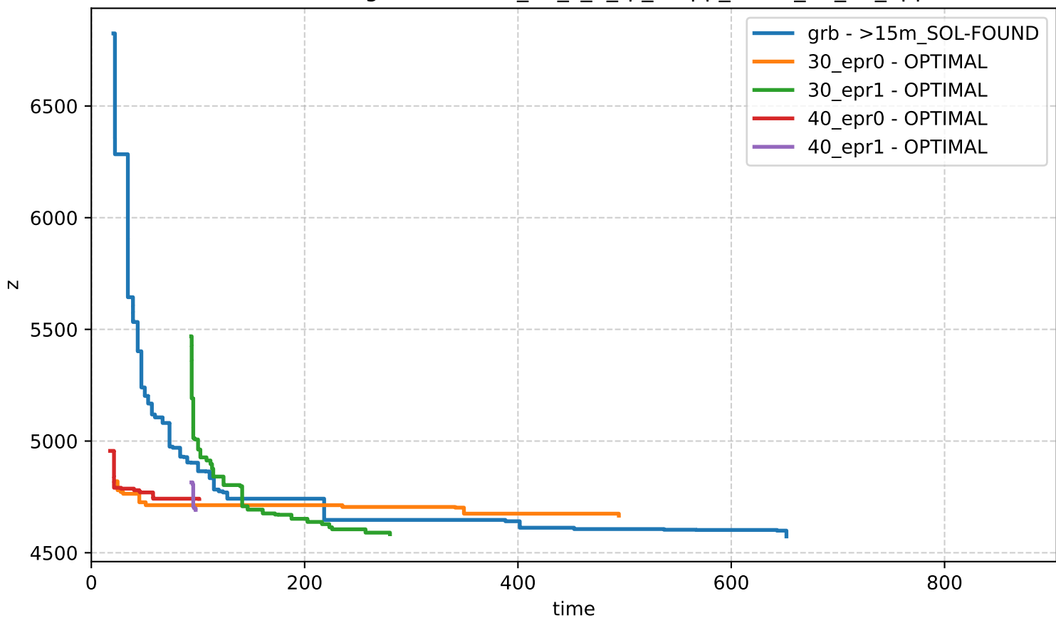
Bound Profiling - network-n_60_s_1_rp_0-app_set-id_38_17_apps
