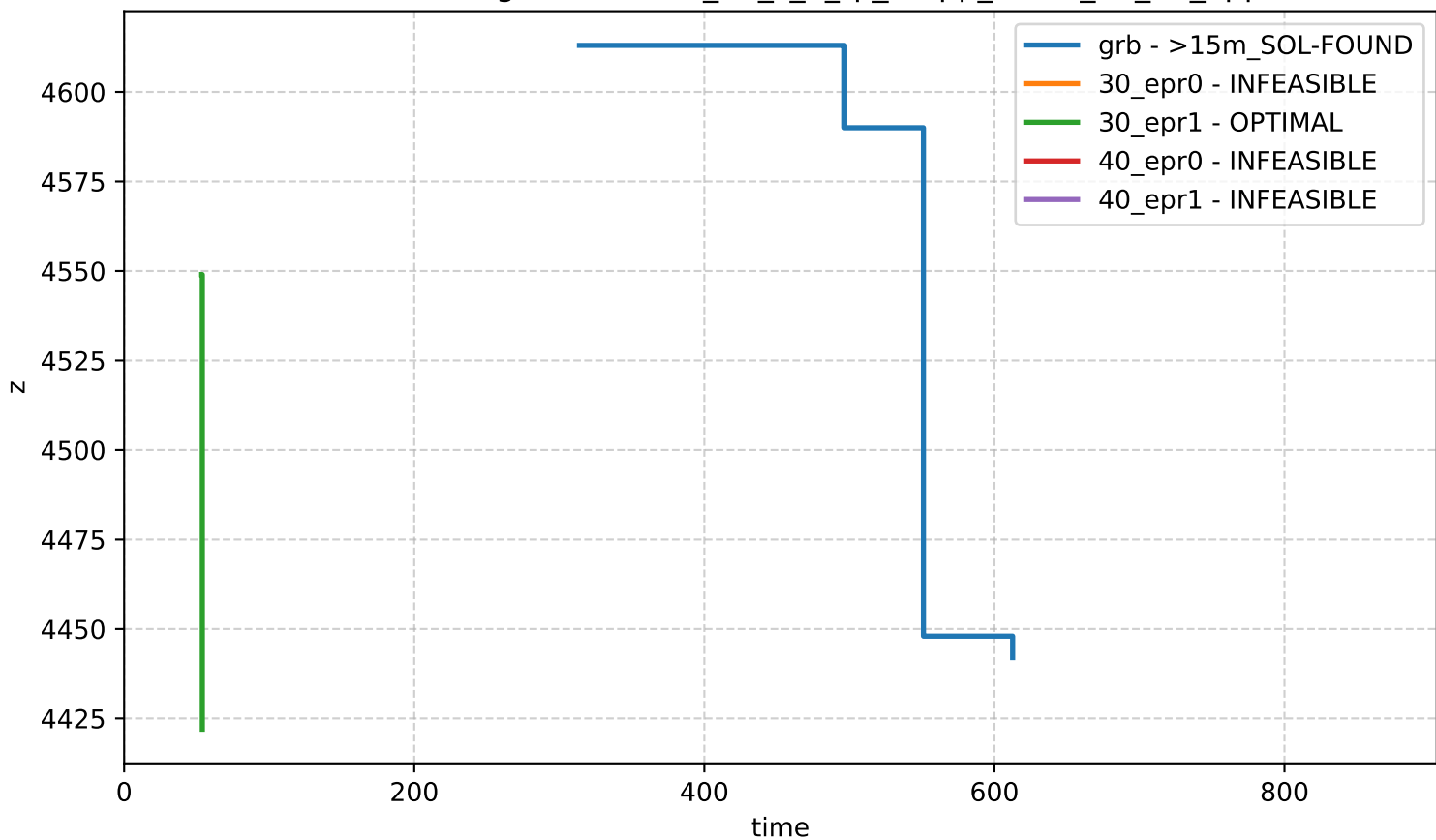
Bound Profiling - network-n_40_s_2_rp_0-app_set-id_33_16_apps
