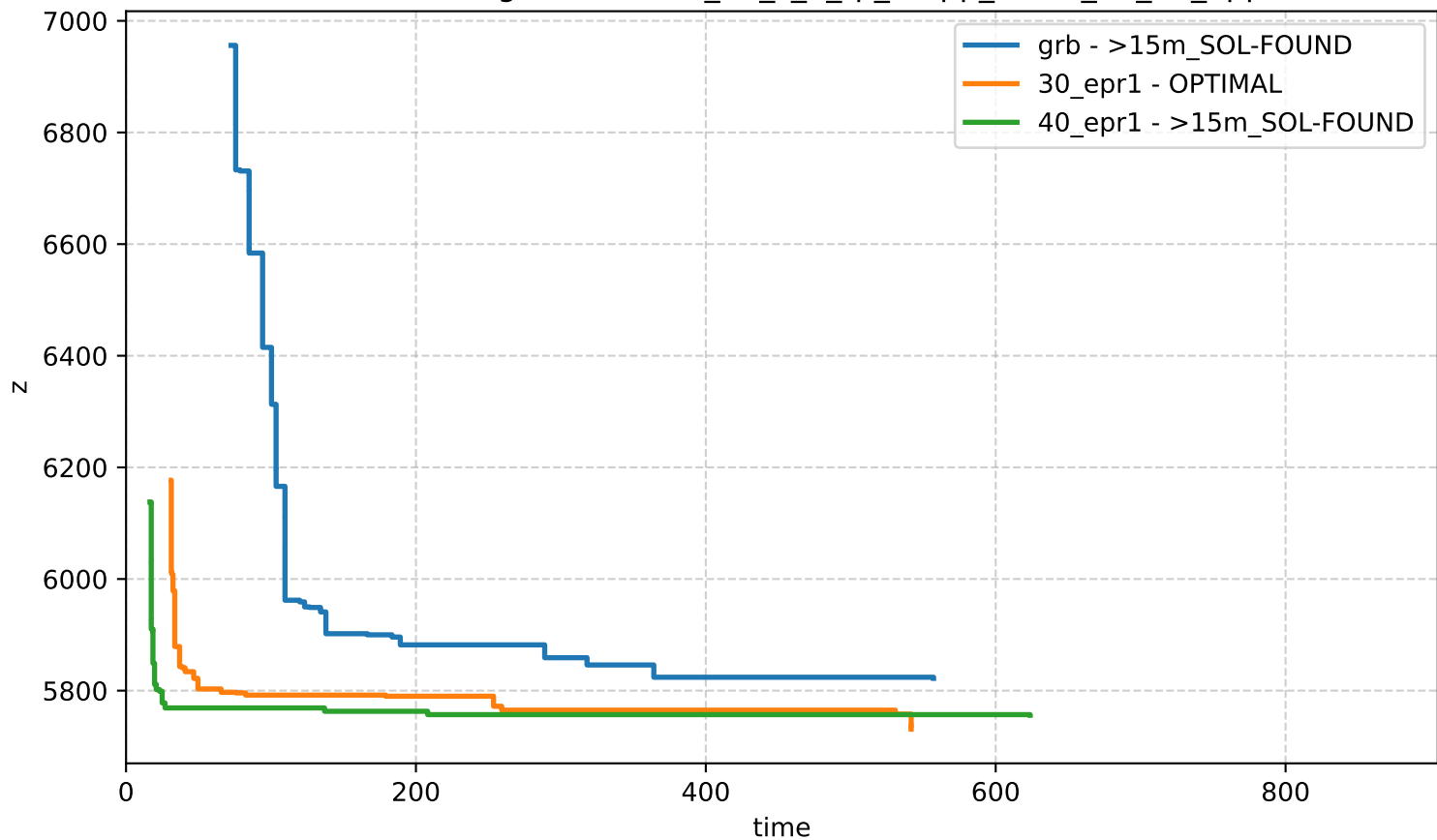
Bound Profiling - network-n_60_s_0_rp_0-app_set-id_55_23_apps
