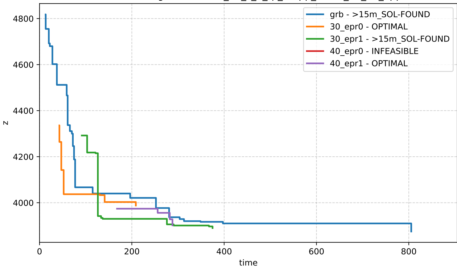
Bound Profiling - network-n 50 s 2 rp 0-app set-id 37 17 apps
