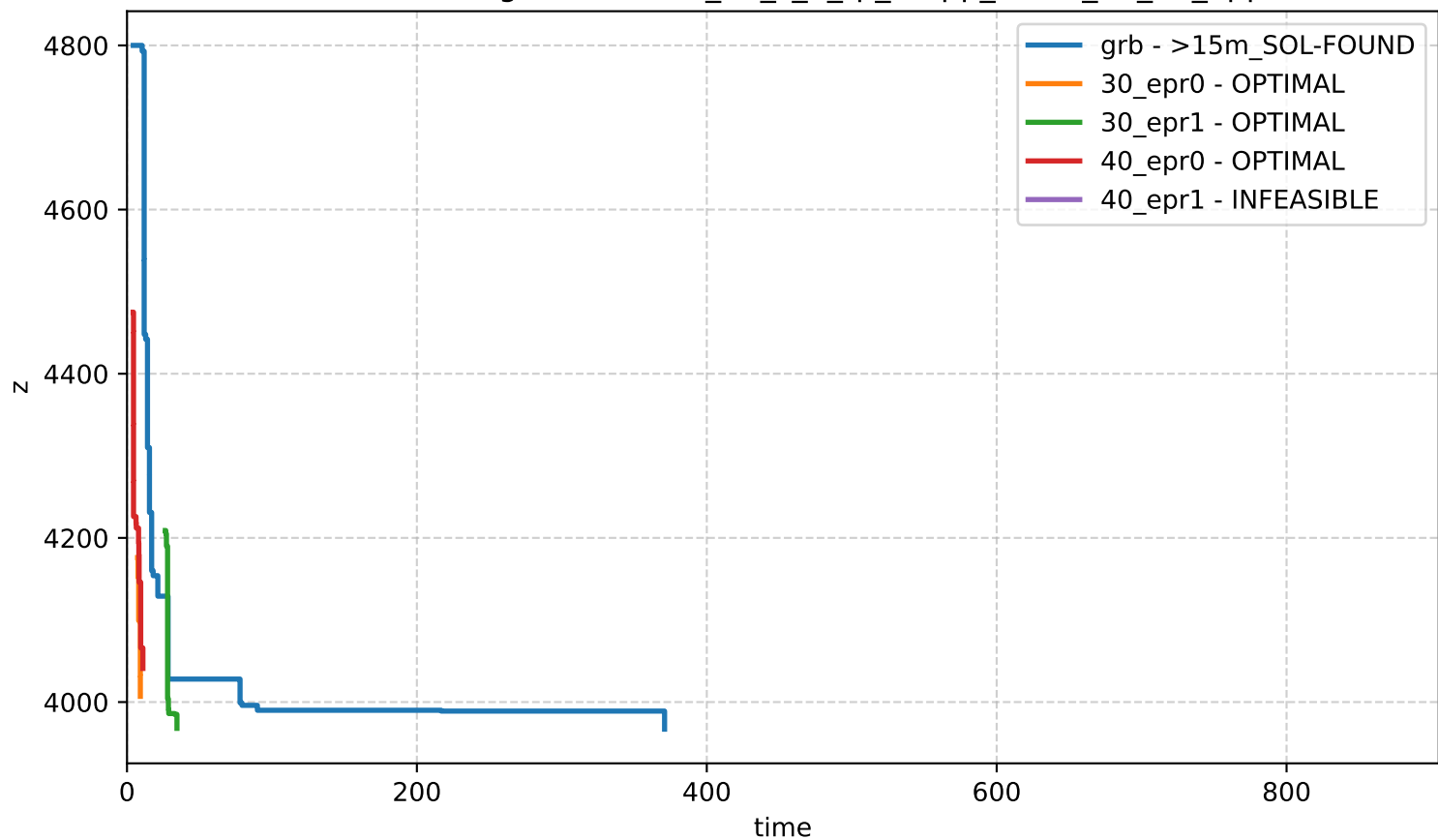
Bound Profiling - network-n_40_s_1_rp_0-app_set-id_34_16_apps
