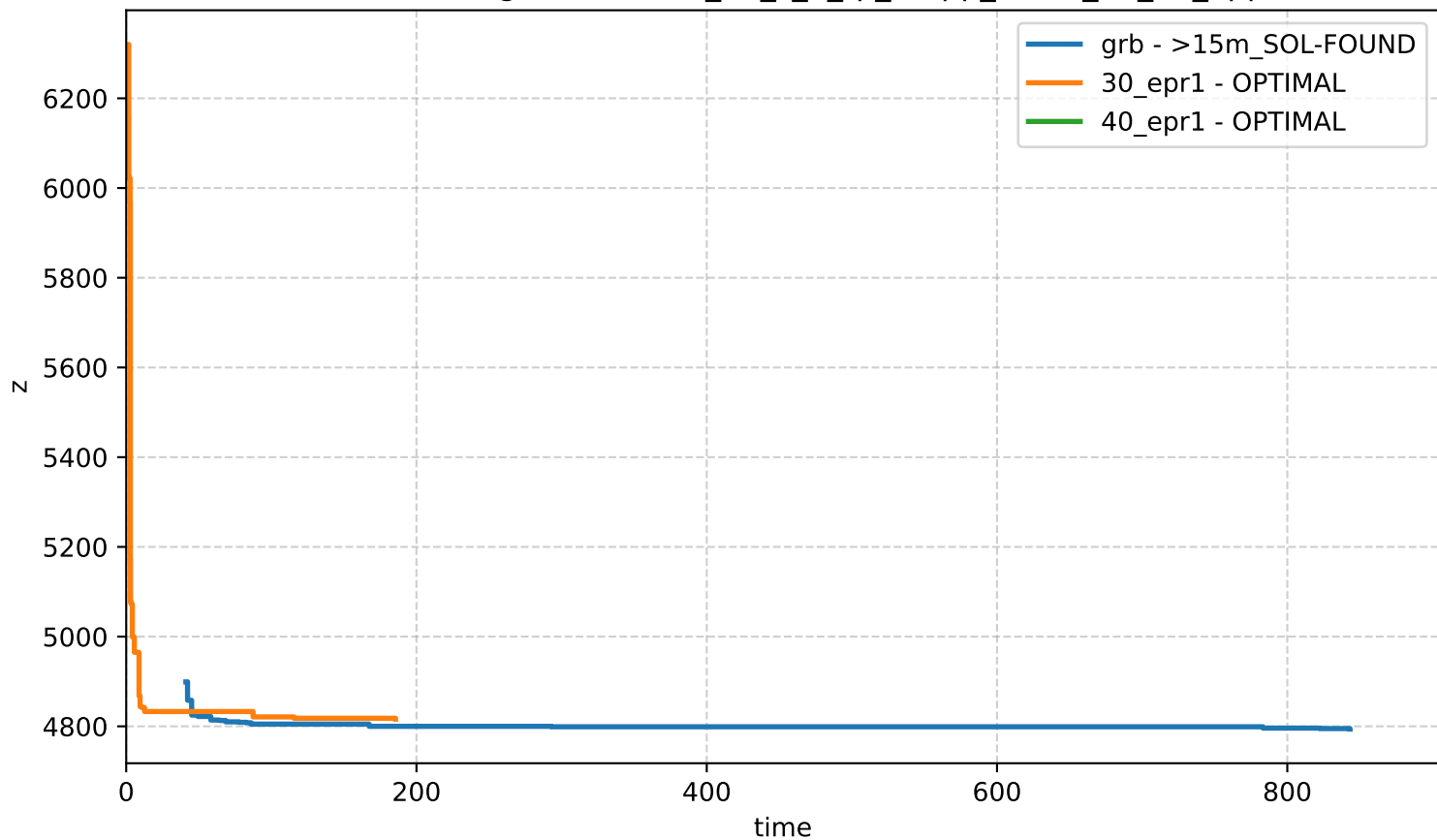
Bound Profiling - network-n_60_s_0_rp_0-app_set-id_42_19_apps
