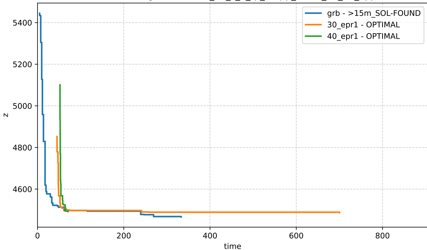
Bound Profiling - network-n_60_s_2_rp_0-app_set-id_42_19_apps
