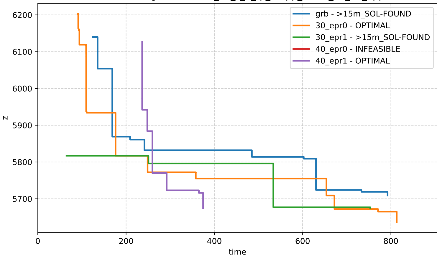
Bound Profiling - network-n_60_s_1_rp_0-app_set-id_47_20_apps
