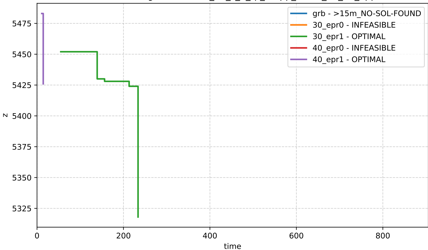
Bound Profiling - network-n_50_s_0_rp_0-app_set-id_41_18_apps
