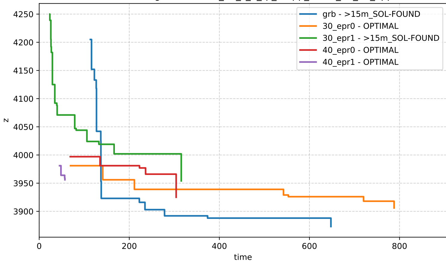
Bound Profiling - network-n_40_s_1_rp_0-app_set-id_37_17_apps
