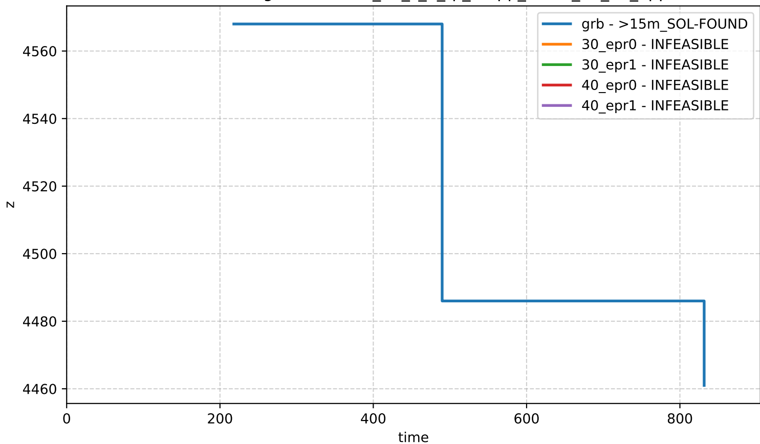
Bound Profiling - network-n_40_s_1_rp_0-app_set-id_31_15_apps
