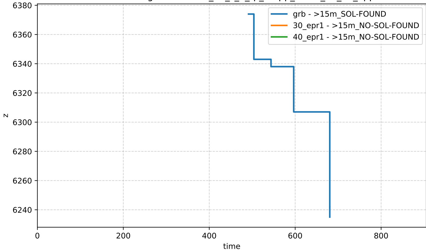
Bound Profiling - network-n_60_s_2_rp_0-app_set-id_59_24_apps
