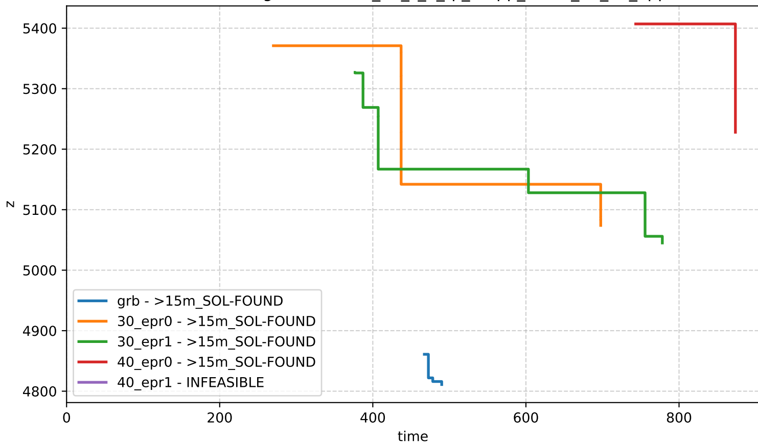
Bound Profiling - network-n_50_s_0_rp_0-app_set-id_48_21_apps
