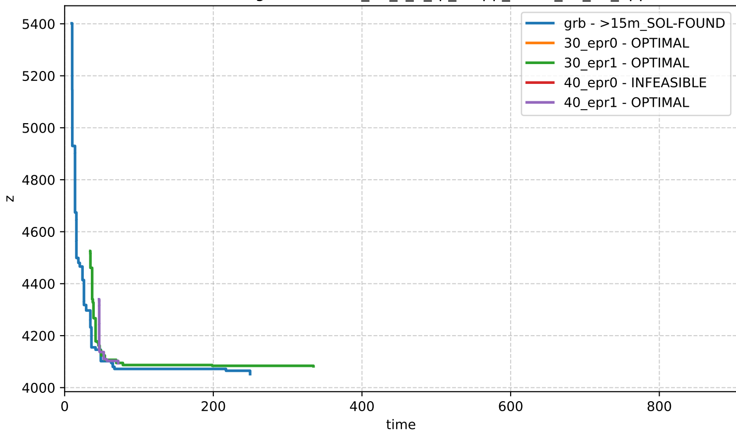
Bound Profiling - network-n_50_s_1_rp_0-app_set-id_31_15_apps
