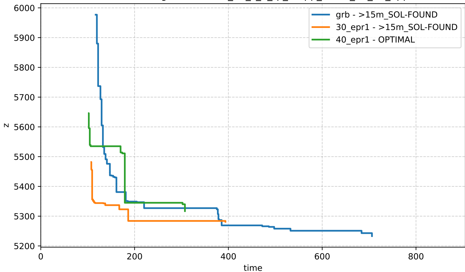
Bound Profiling - network-n_60_s_0_rp_0-app_set-id_49_21_apps
