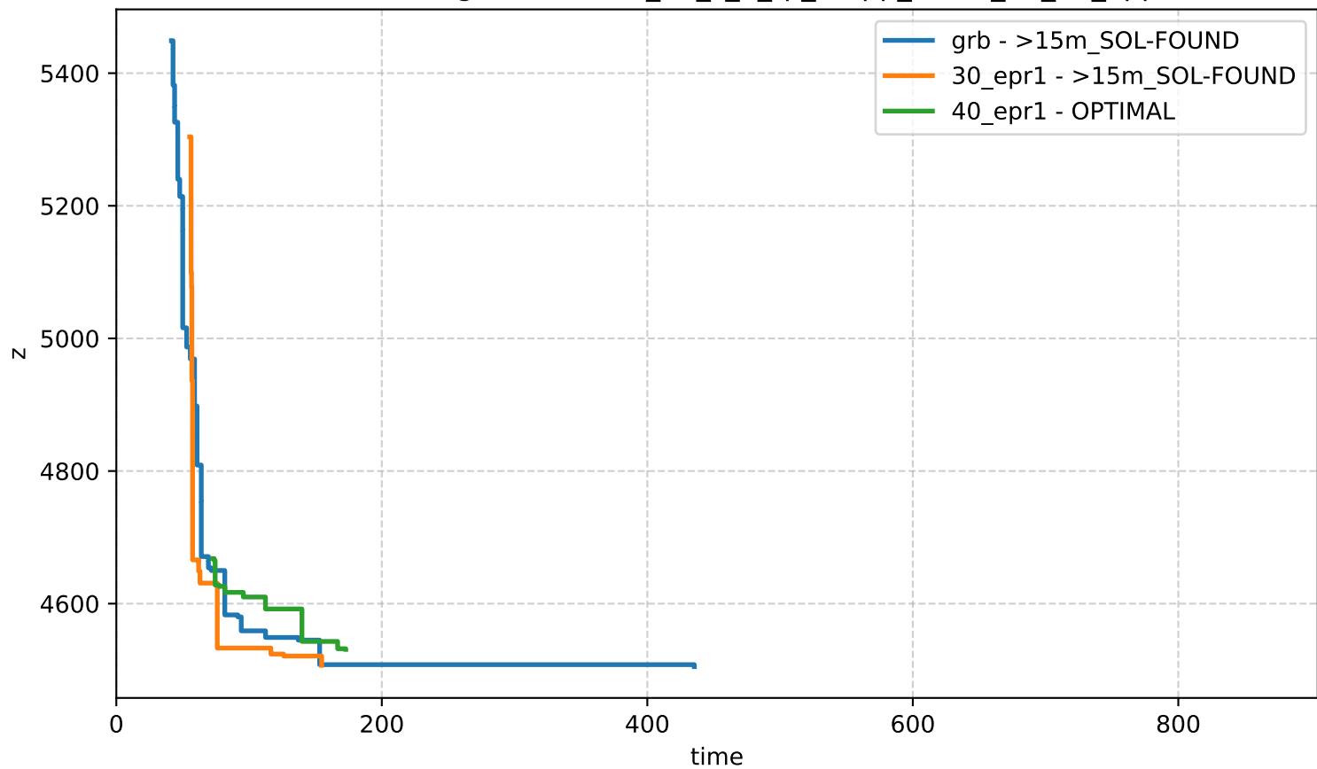
Bound Profiling - network-n_60_s_2_rp_0-app_set-id_43_19_apps
