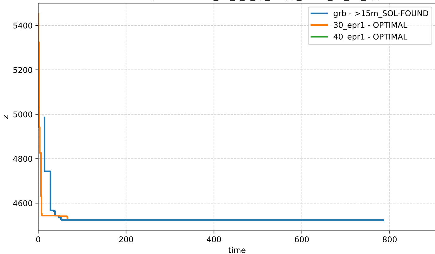
Bound Profiling - network-n_60_s_0_rp_0-app_set-id_39_18_apps
