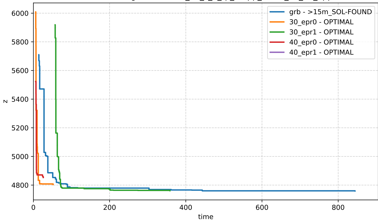
Bound Profiling - network-n_60_s_0_rp_0-app_set-id_40_18_apps
