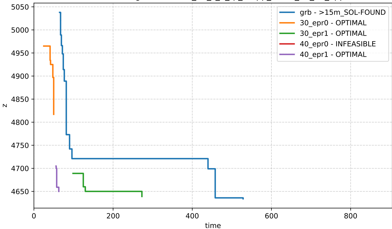
Bound Profiling - network-n_50_s_1_rp_0-app_set-id_35_16_apps
