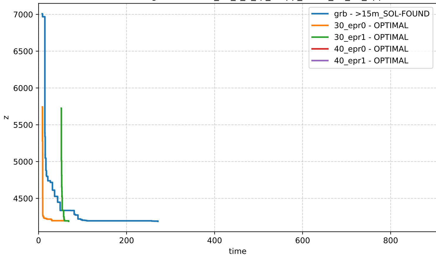
Bound Profiling - network-n_60_s_0_rp_0-app_set-id_38_17_apps
