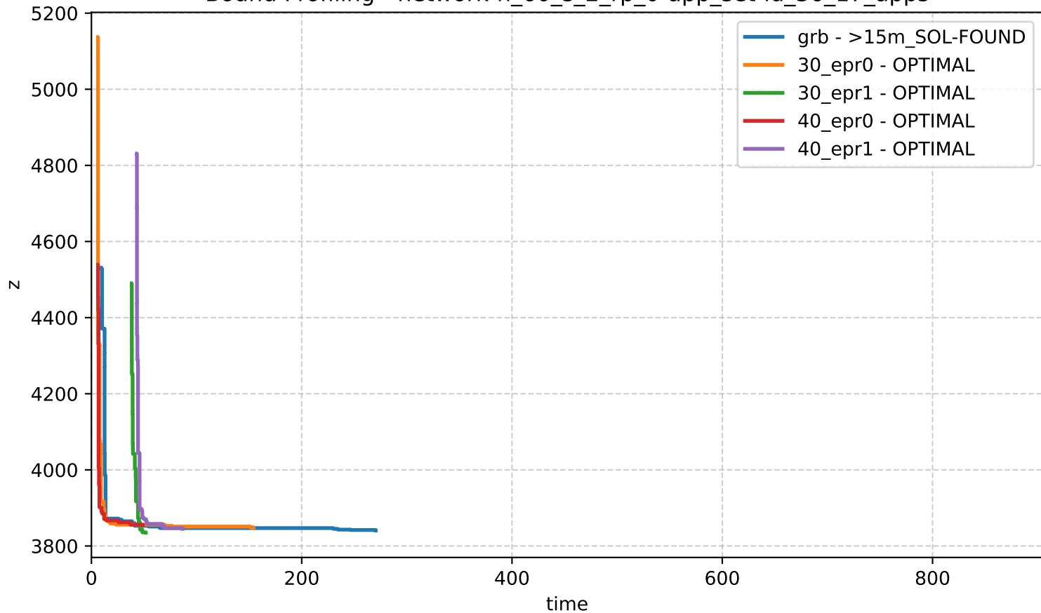
Bound Profiling - network-n_60_s_2_rp_0-app_set-id_36_17_apps
