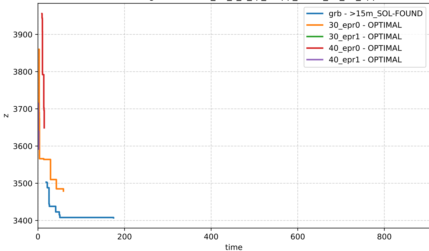
Bound Profiling - network-n_30_s_1_rp_0-app_set-id_33_16_apps
