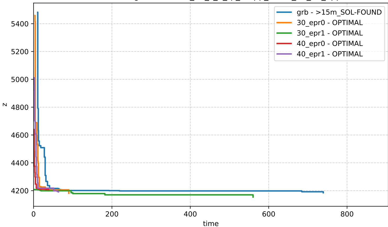
Bound Profiling - network-n_60_s_1_rp_0-app_set-id_36_17_apps
