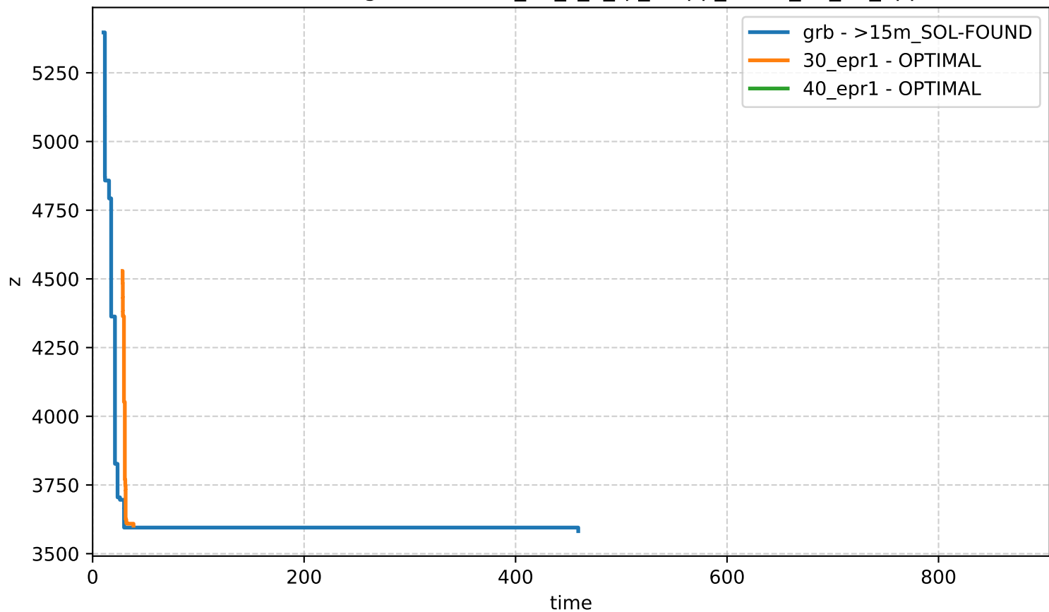
Bound Profiling - network-n_50_s_1_rp_0-app_set-id_33_16_apps
