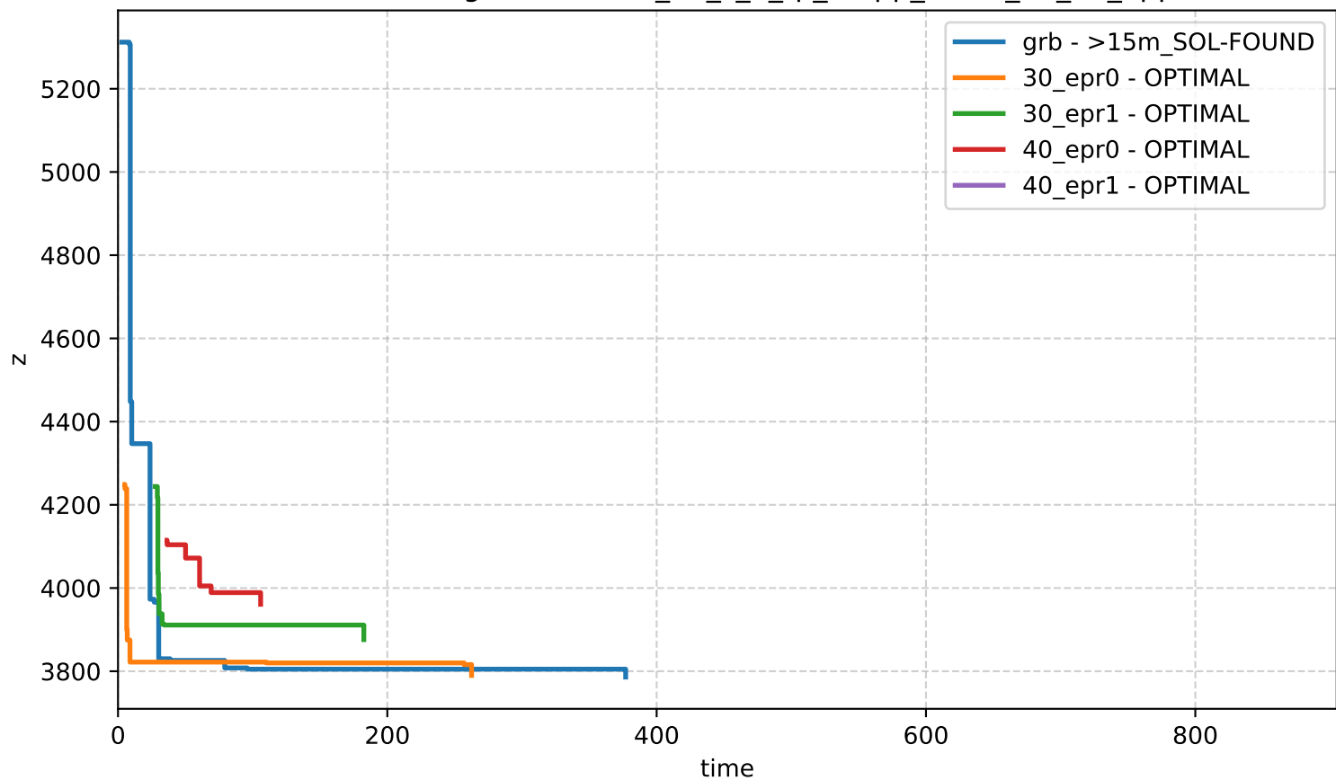
Bound Profiling - network-n_50_s_2_rp_0-app_set-id_34_16_apps
