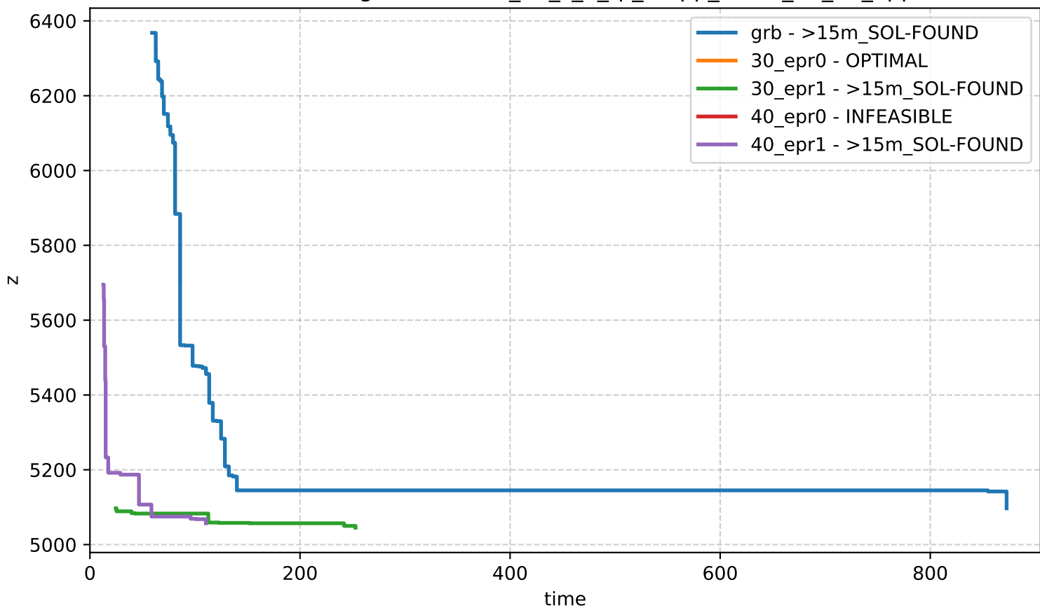
Bound Profiling - network-n_60_s_1_rp_0-app_set-id_51_22_apps
