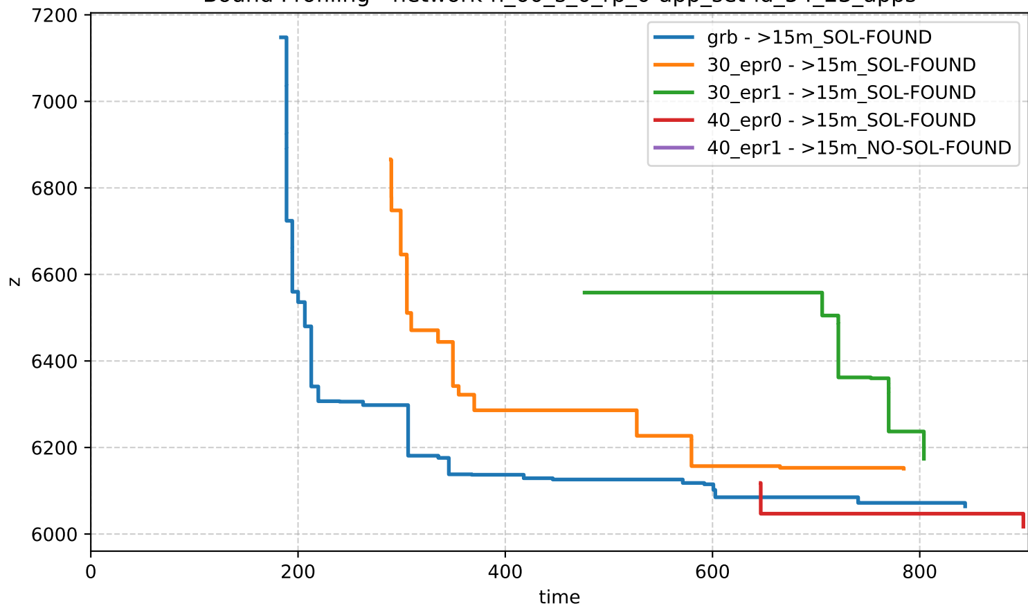
Bound Profiling - network-n_60_s_0_rp_0-app_set-id_54_23_apps
