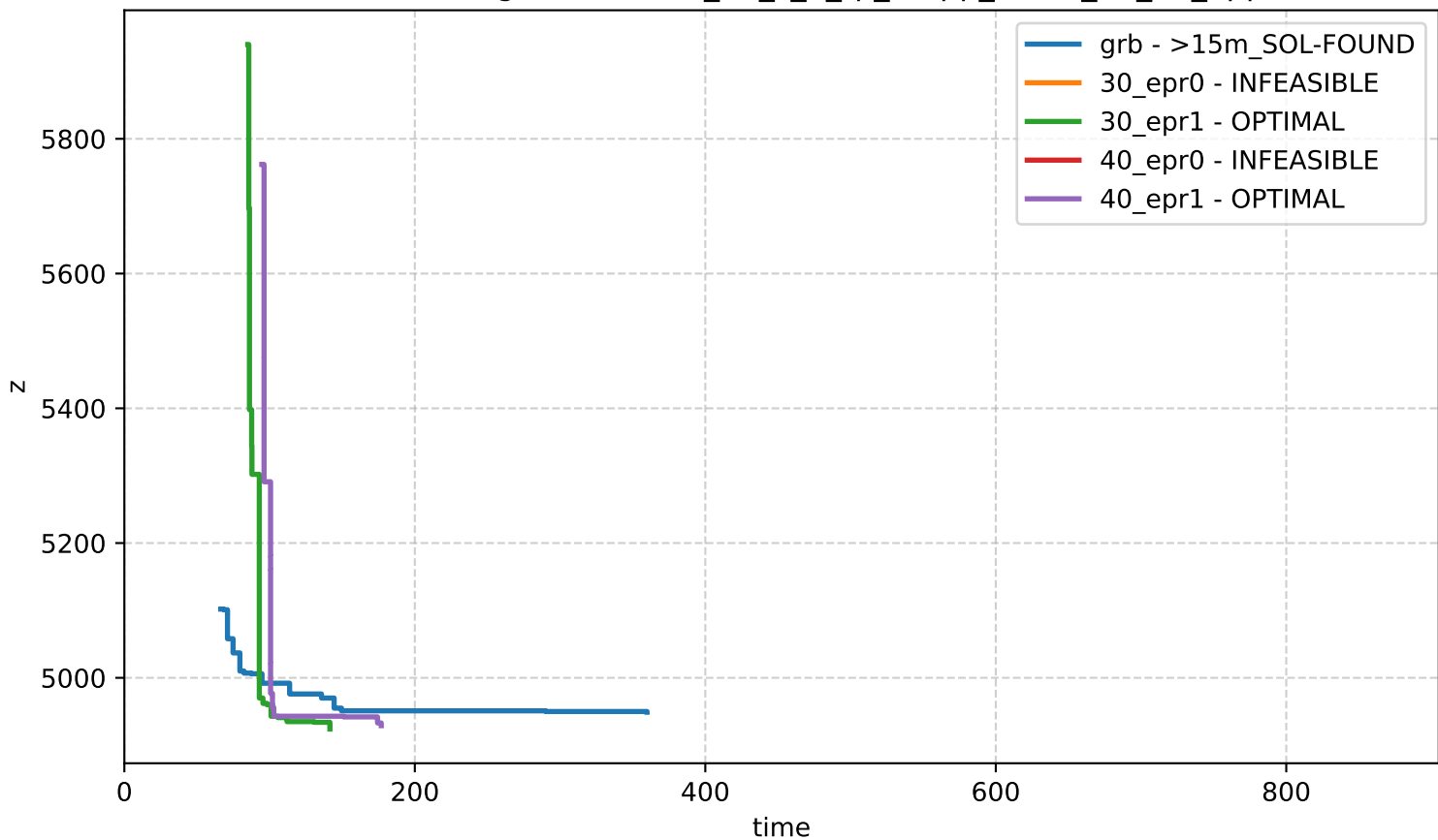
Bound Profiling - network-n_60_s_0_rp_0-app_set-id_45_20_apps
