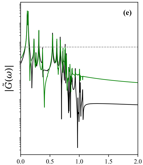
LiH (6-31G, R=1.5 \text{ \AA} , n_o=10 , n_e=4 )
