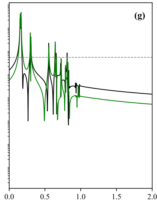
LiH (6-31G, R=1.5 \text{ \AA} , n_o=10 , n_e=4 )
