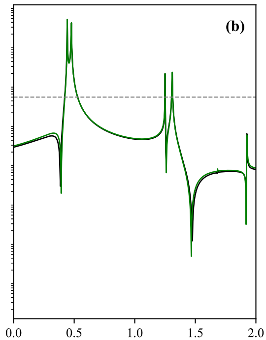
LiH (CC-PVDZ, R=1.5 \text{ \AA} , n_o=16 , n_e=4 )
