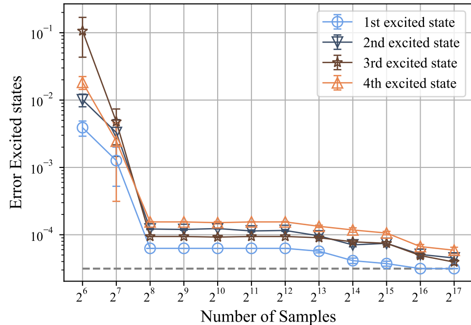
HCl (STO-6G, R=1.2 \text{ \AA} , n_o = 10 , n_e = 18 )
