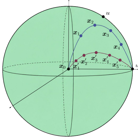
Figure 3.2: Intuitively, uniform fixed-share helps the learner revisit downweighted regions through uniform draws, whose mean is the barycenter of \mathcal{K} . From the common initialization \mathbf{x}_0 , the schematic trajectories \mathbf{x}'_1, \dots, \mathbf{x}'_5 (bordeaux, with fixed-share) and \mathbf{x}_1, \dots, \mathbf{x}_4 (blue, without fixed-share) initially move towards the comparator \mathbf{u} and then turn towards \mathbf{u}' after a loss change. The fixed-share trajectory shows a conservative response to the initial losses, reflecting the goal of attaining lower interval regret and comparable static regret.
