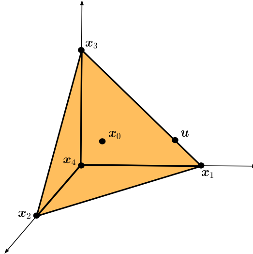
Figure 2.1: A simplex illustrates the distinction between multi-armed and linear bandits. In the multi-armed setting, the vertices correspond to the arms and are the only playable actions, while a point in their convex hull represents a distribution over them. The coefficients of the convex combination specify the sampling probabilities; the barycenter corresponds to the uniform distribution. In the linear setting, the entire simplex forms the action set: every convex combination of its vertices, including \mathbf{u} , is itself a playable action.
