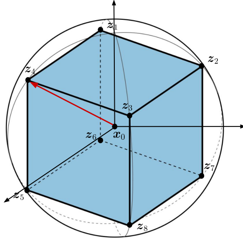
Figure 3.1: Löwner position for a cubic decision set in \mathbb{R}^3 . The transformed set \mathcal{L}(\mathcal{K}) is inscribed in the Euclidean unit ball \mathbb{B}_2^3 , which represents its minimum volume enclosing ellipsoid. The vertices \mathbf{z}_1, \dots, \mathbf{z}_8 are contact points with \partial \mathbb{B}_2^3 and support a probability distribution yielded by \pi_1, \dots, \pi_m . The arrow in red illustrates an exploratory action toward a contact point, starting from \mathbf{x}_0 (the barycenter of \mathbb{B}_2^3 and the coordinate origin). This construction encourages exploration on geometrically informative boundary directions.
