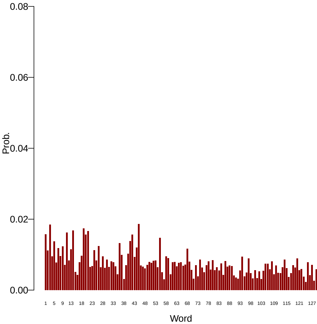
Topic: 18
