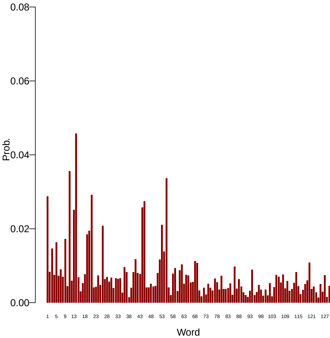
Topic: 16
