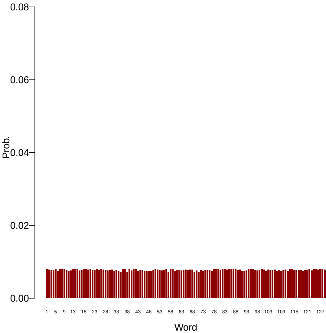
Topic: 37
