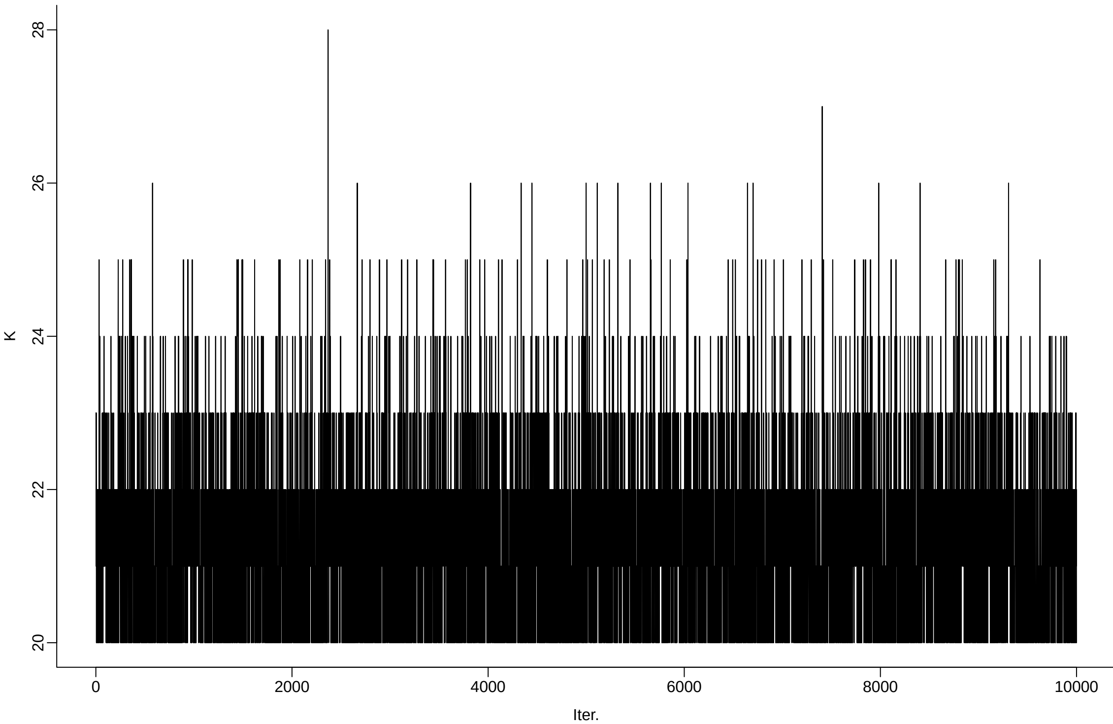
cfg006_r10_delta_1e00_beta0_1e00_gamma0_1em02_sigma0_1em01 | Total number of distinct topics
