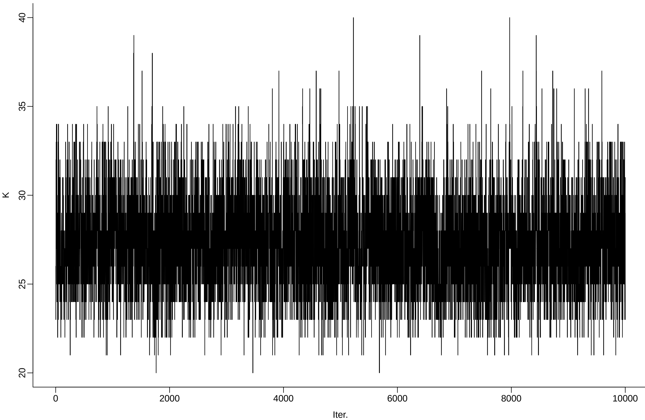
cfg010_r10_delta_1e00_beta0_1em01_gamma0_1em01_sigma0_1em01 | Total number of distinct topics
