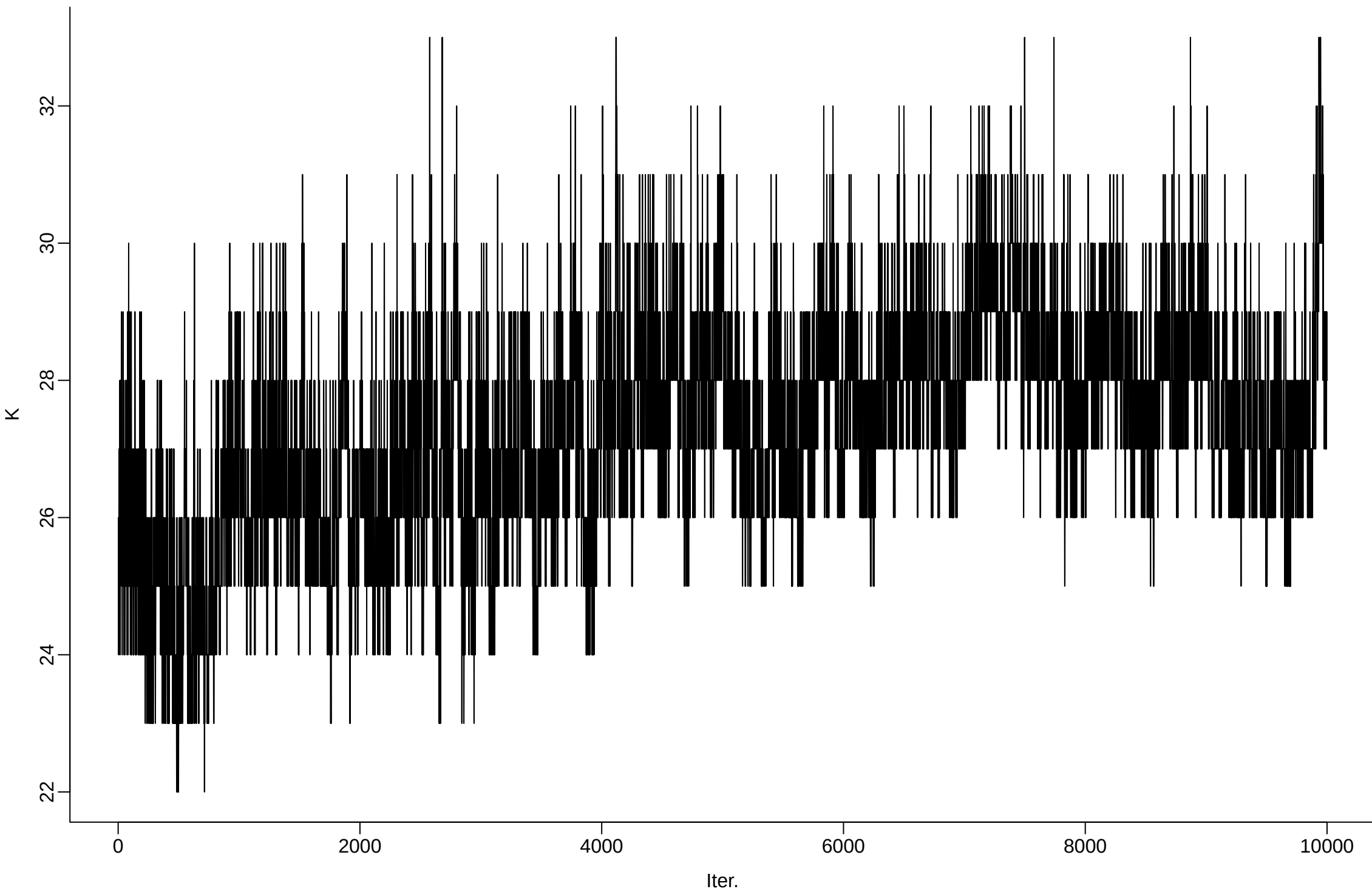
cfg017_r10_delta_1em04_beta0_1e00_gamma0_1em02_sigma0_5em01 | Total number of distinct topics
