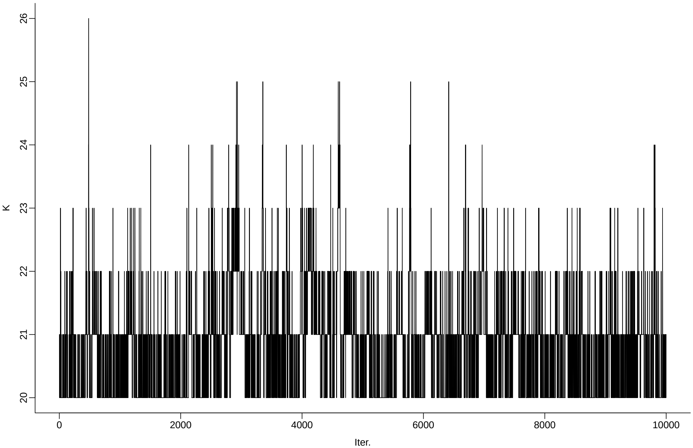
cfg025_r10_delta_1em04_beta0_1em02_gamma0_1em02_sigma0_9em01 | Total number of distinct topics
