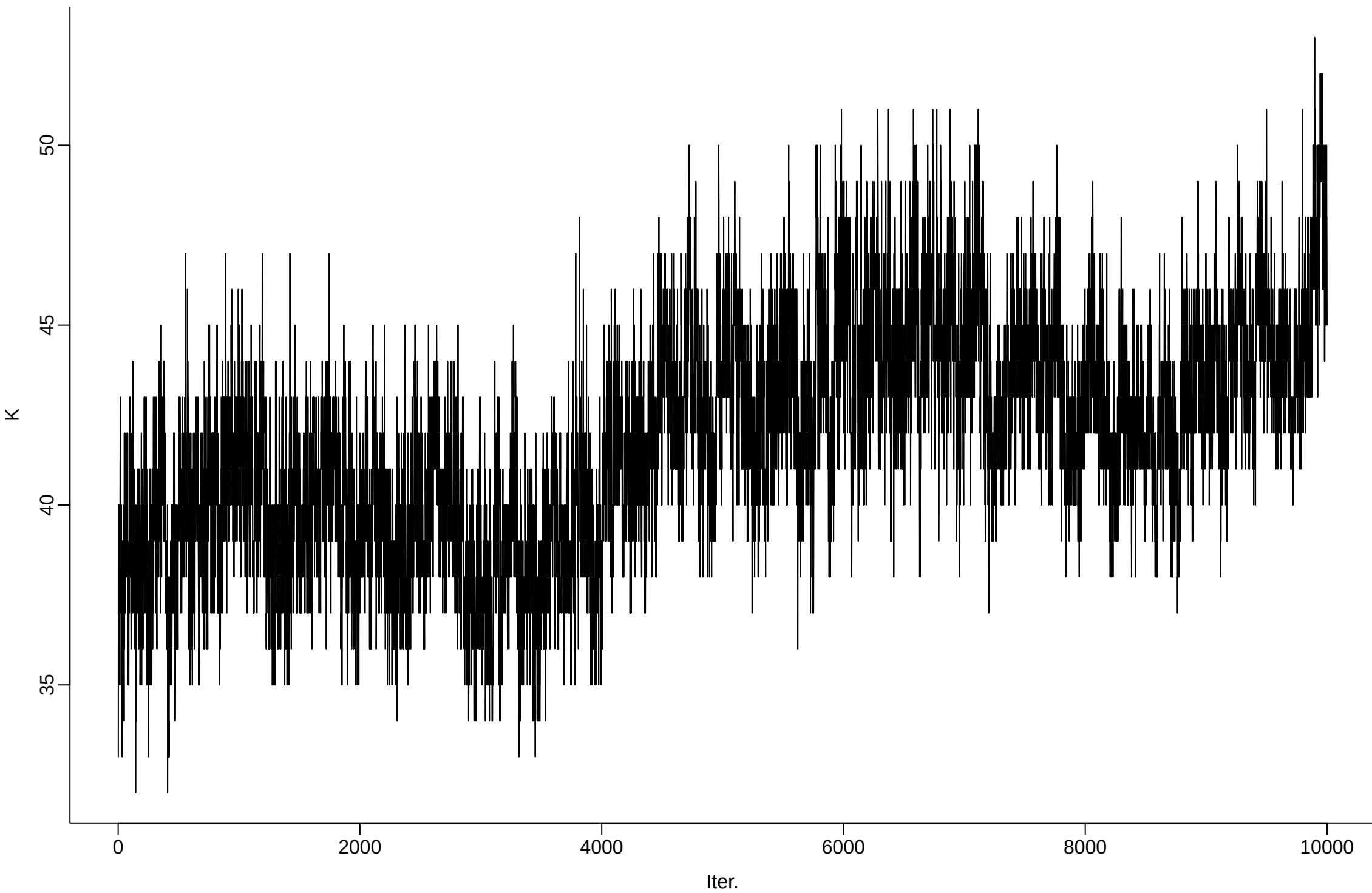
cfg035_r10_delta_1e04_beta0_1e00_gamma0_1e01_sigma0_9e01 | Total number of distinct topics
