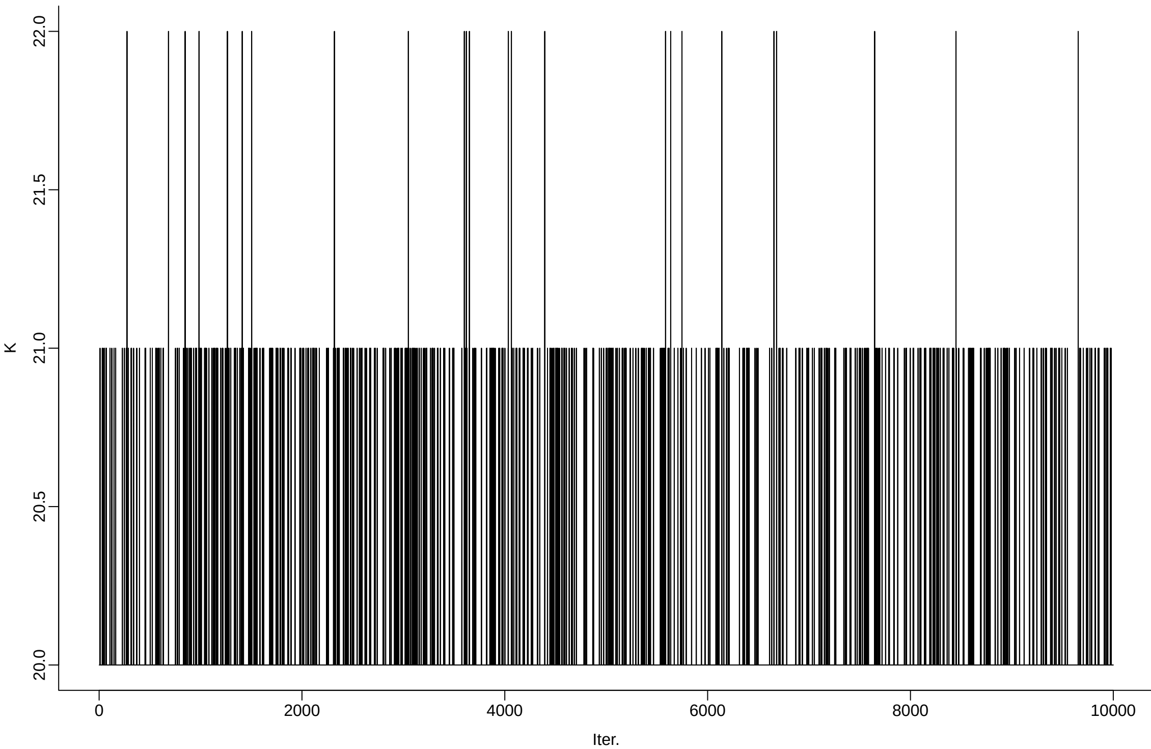
cfg029_r10_delta_1em03_beta0_1e00_gamma0_1em03_sigma0_1em01 | Total number of distinct topics
