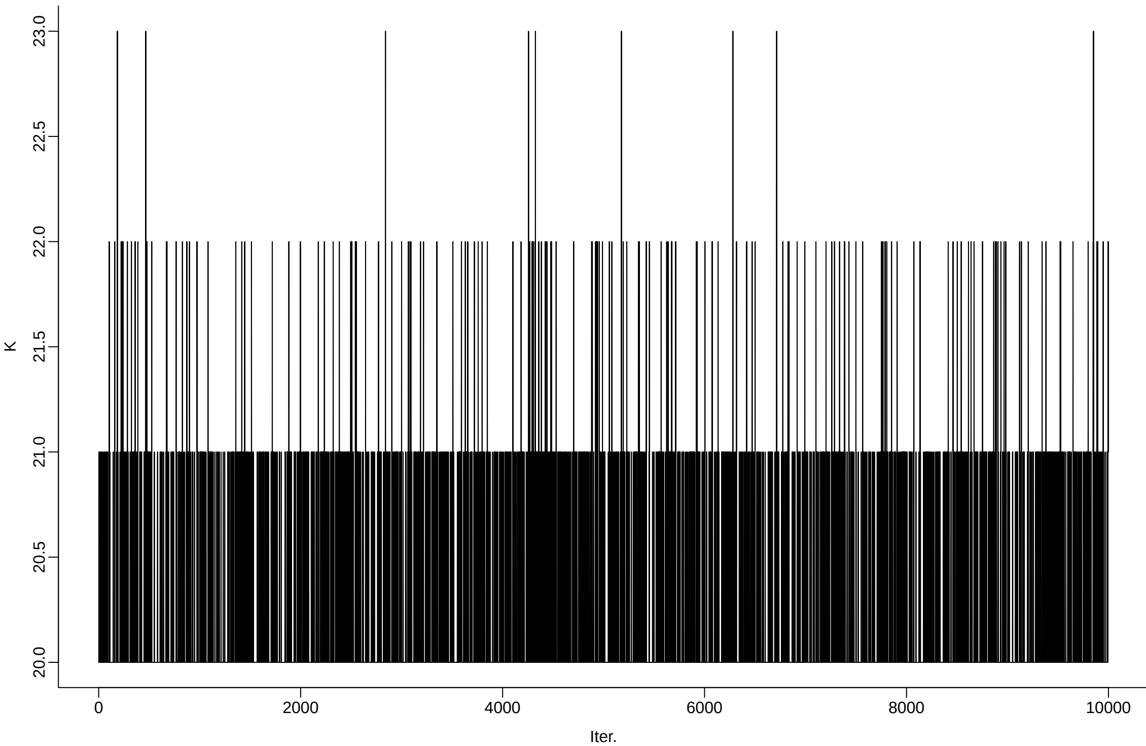
cfg041_r10_delta_1em03_beta0_1em01_gamma0_1em02_sigma0_1em01 | Total number of distinct topics
