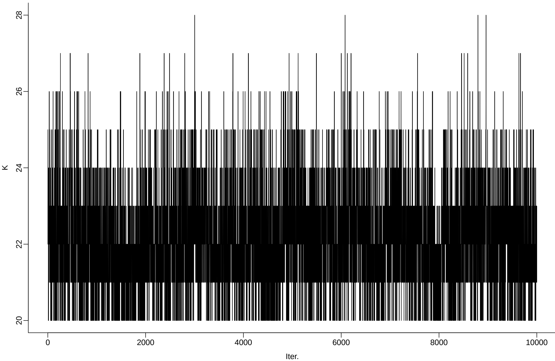
cfg047_r10_delta_1em03_beta0_1em04_gamma0_1em01_sigma0_1em01 | Total number of distinct topics
