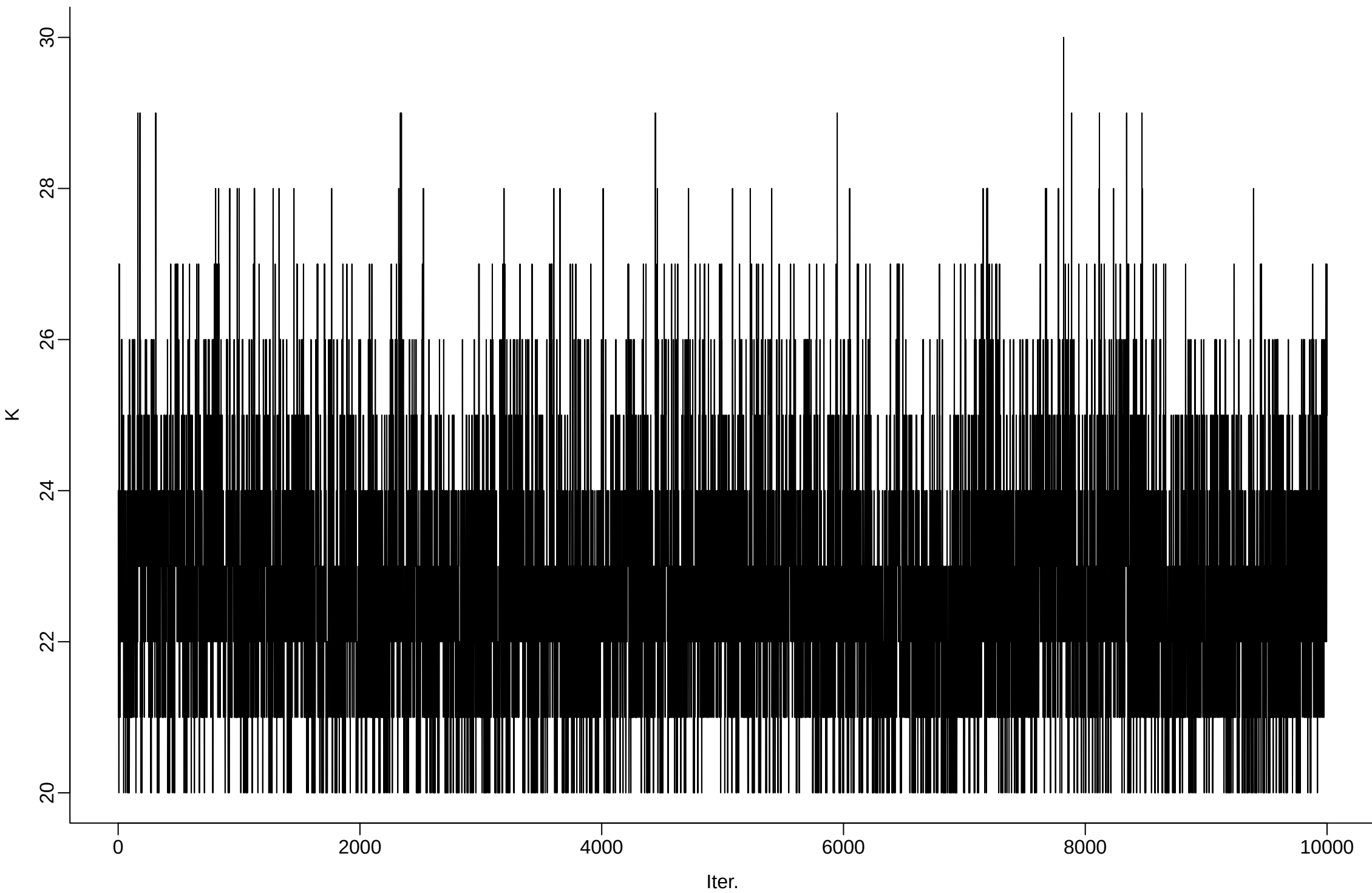
cfg057_r10_delta_1em02_beta0_1em01_gamma0_1em01_sigma0_1em01 | Total number of distinct topics
