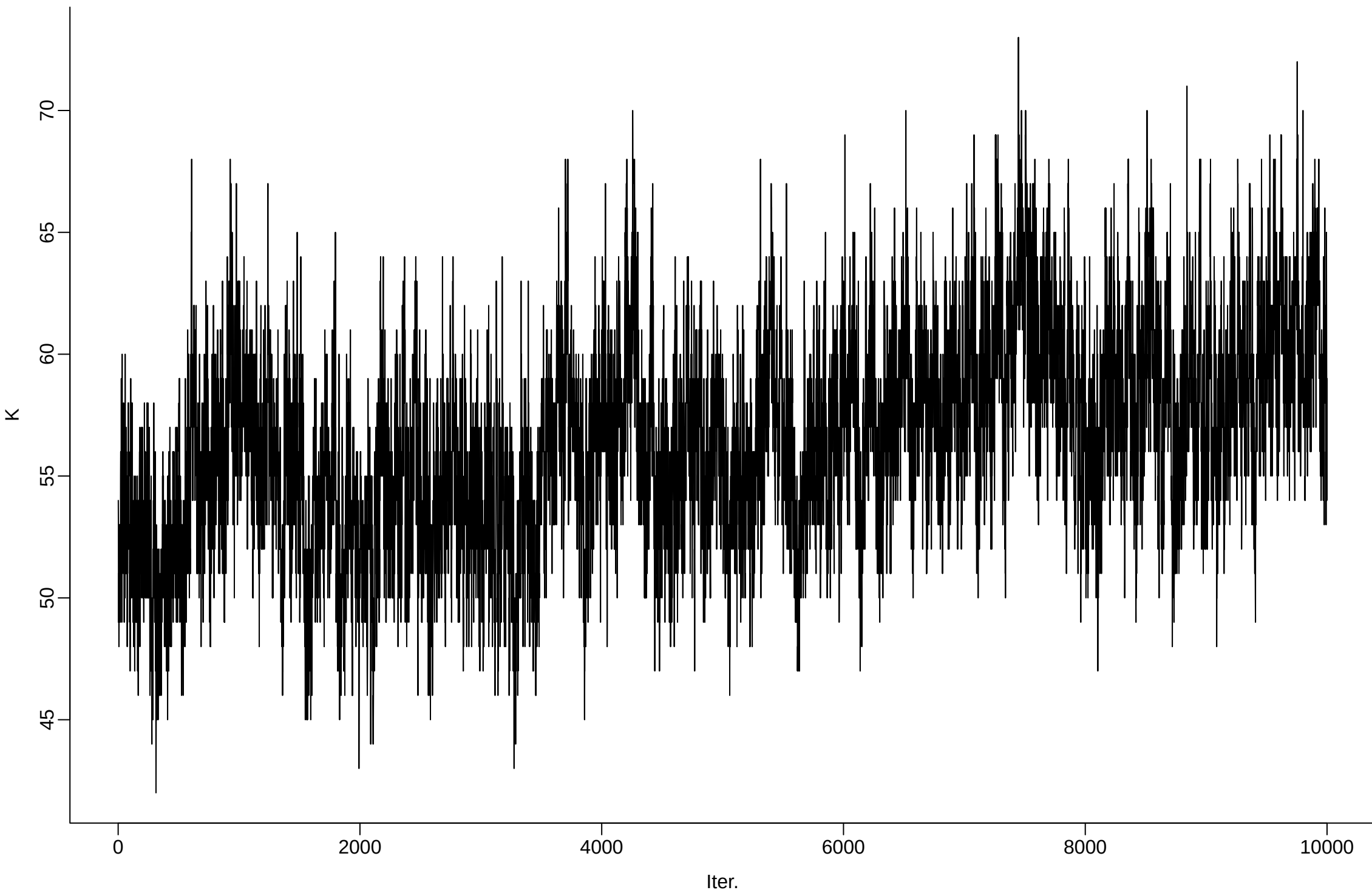
cfg065_r10_delta_1em03_beta0_1em03_gamma0_1e00_sigma0_1em01 | Total number of distinct topics
