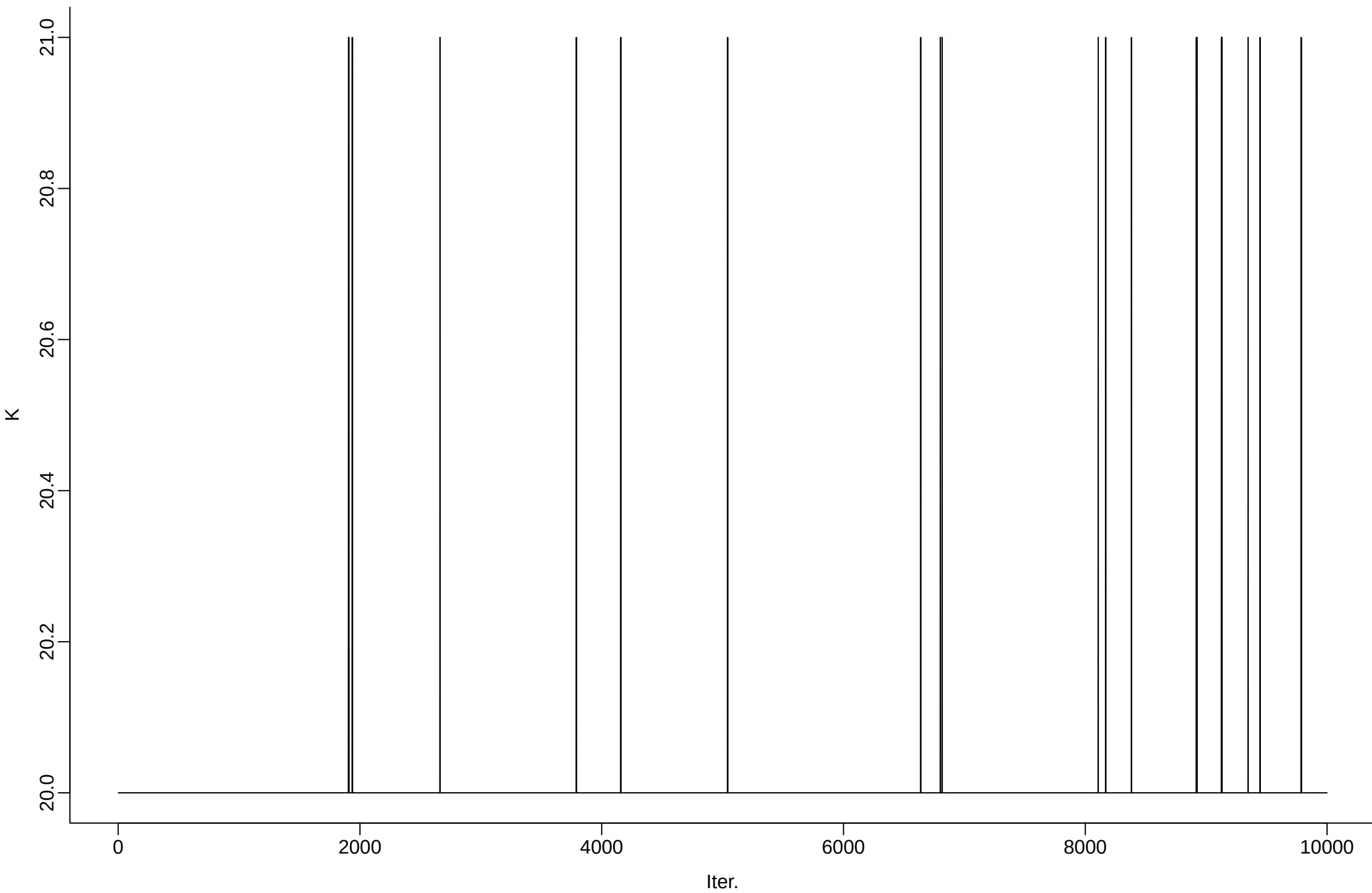
cfg080_r10_delta_1em03_beta0_1em03_gamma0_1em04_sigma0_2p5em01 | Total number of distinct topics
