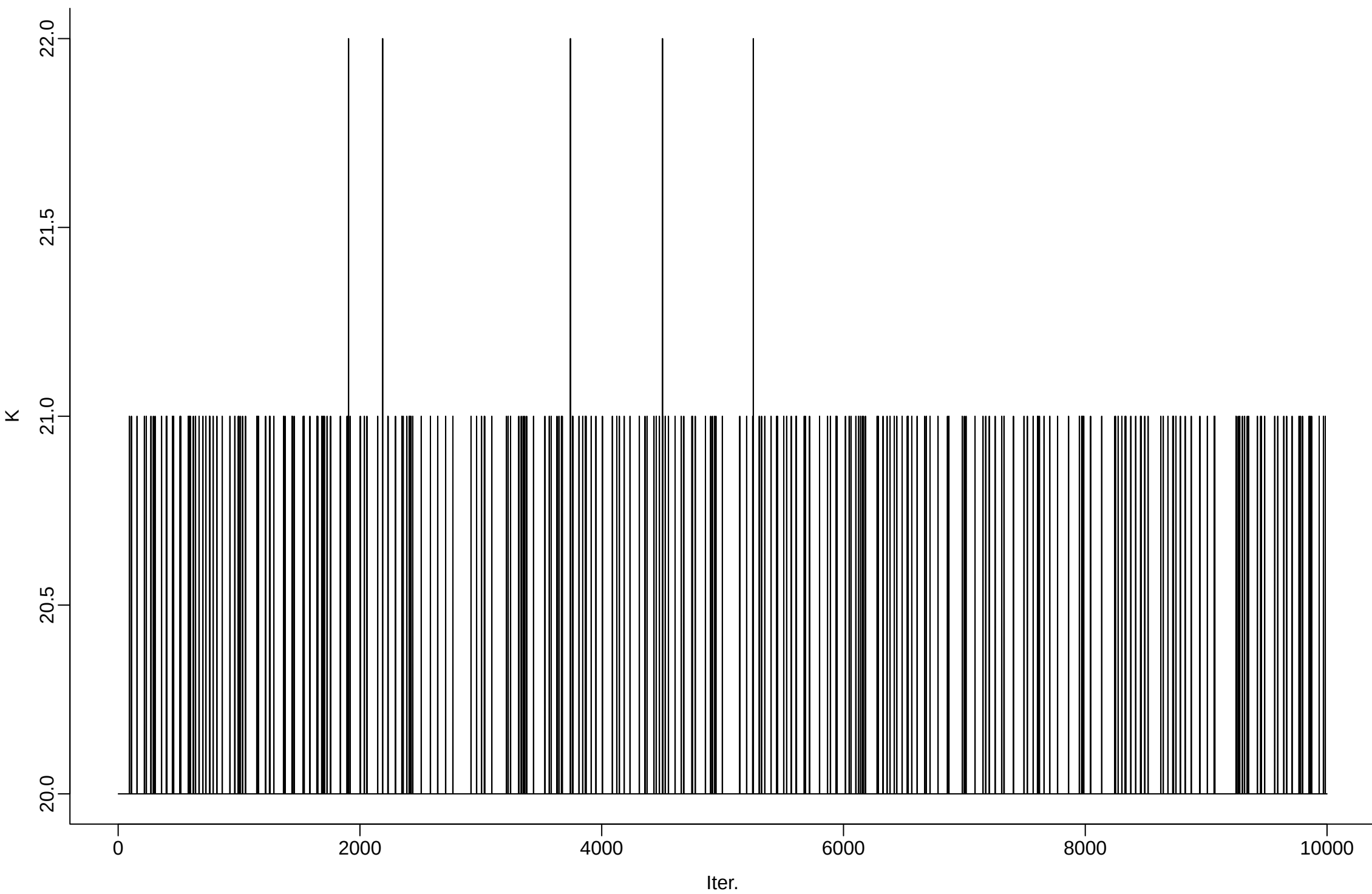
cfg102_r10_delta_1em02_beta0_1em01_gamma0_1em03_sigma0_2p5em01 | Total number of distinct topics
